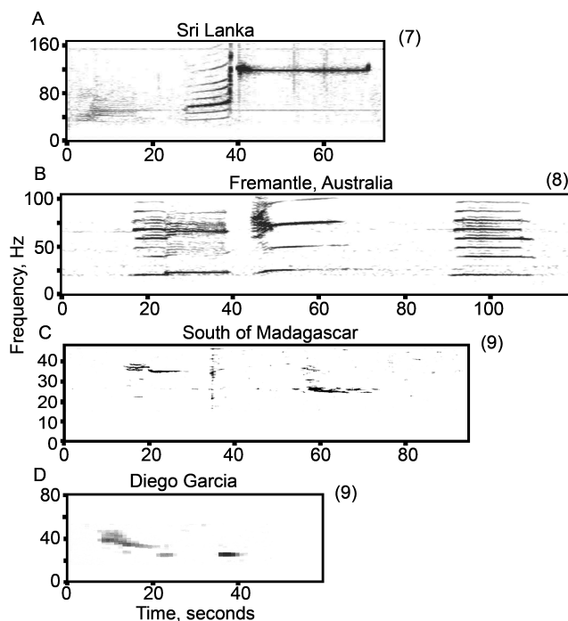
Fig. 5. Blue whale songs for: (A) North Indian Ocean – Sri Lanka, recorded April, 1984 within 5 miles of the entrance to Trincomalee Harbour (Alling and Payne, 1987). Spectrogram produced from archival tape at the British Library, Natural Sound Archive, London, (B) Southeast Indian Ocean – Fremantle, recorded west of Perth, Australia (courtesy of R. McCauley), (C) Southwest Indian Ocean – Madagascar, recorded December 1996, south of the Madagascar Plateau (after Ljungblad et al. , 1998), and (D) Southwest Indian Ocean – Diego Garcia, recorded October 2000, south of Diego Garcia, by the Comprehensive Test Ban Treaty Organisation. The numbers in brackets refer to song types.
