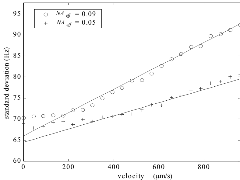
Figure 3. Standard deviation dependence on velocity and NA_{eff} at Doppler angle 77 degree°, the solid line is theoretical curve from equation (11). For NA_{eff} equals 0.09 and 0.05, the background b is 66 and 64.5 Hz, respectively.
