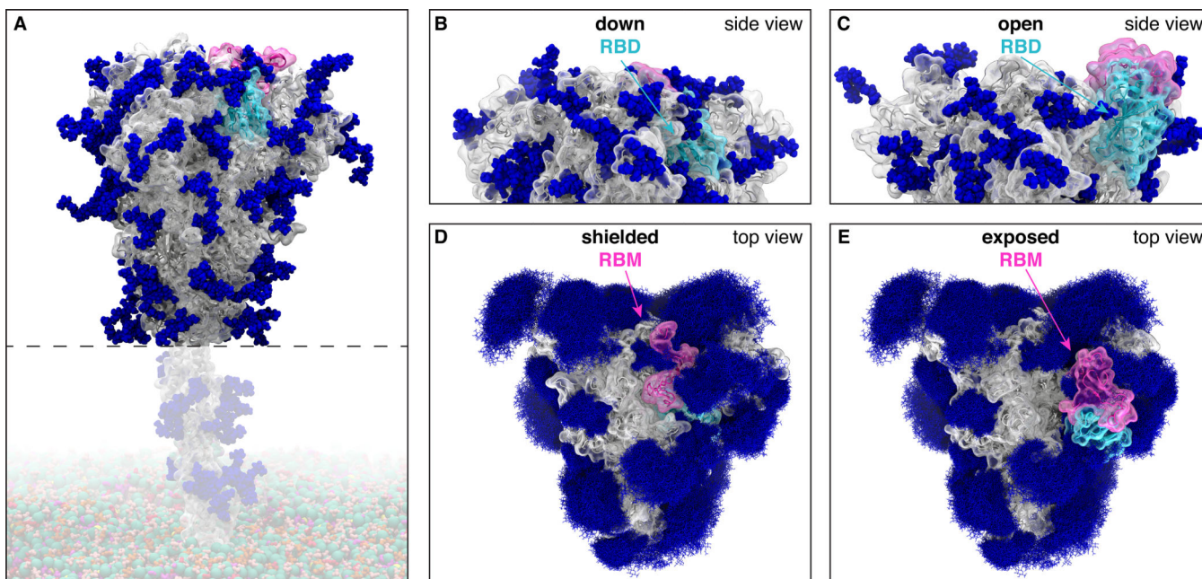
Figure 1. Glycosylated spike RBD “down” and “open” conformations. (A) The SARS-CoV-2 spike head (gray) with glycans (dark blue) as simulated, with the stalk domain and membrane (not simulated here, but shown in transparent for completeness). RBD shown in cyan, receptor binding motif (RBM) in pink. Side view of the “down” (shielded, B) and “open” (exposed, C) RBD. Top view of the closed (shielded, D) and “open” (exposed, E) RBM. Composite image of glycans (dark blue lines) shows many overlapping snapshots of the glycans over the microsecond simulations.
