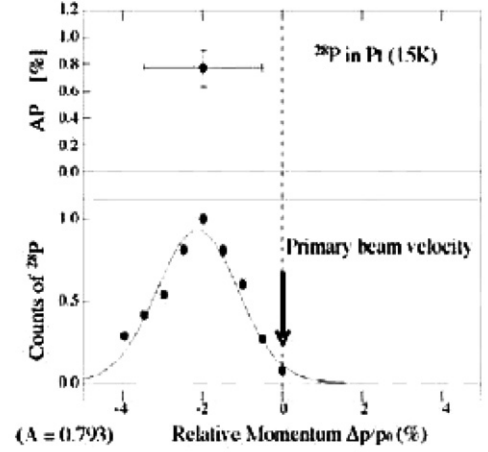
Fig. 1. Polarization as function of momentum.
