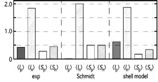
Fig. 3. Decomposition of nuclear spin.
