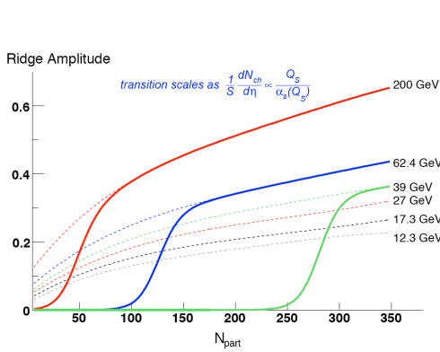
FIG. 44: The un-triggered ridge amplitude as a function of N_{\text{part}} when the transition scale is related to the energy density. The different colored curves represent different \sqrt{s_{NN}} .
