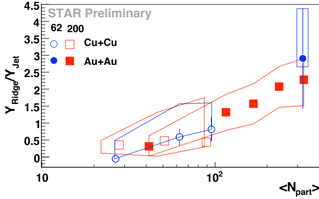
FIG. 48: The Ridge/Jet correlation yield ratio as a function of N_{\text{part}} for Cu+Cu and Au+Au collisions at \sqrt{s_{NN}} = 62 and 200 GeV. From [154].
