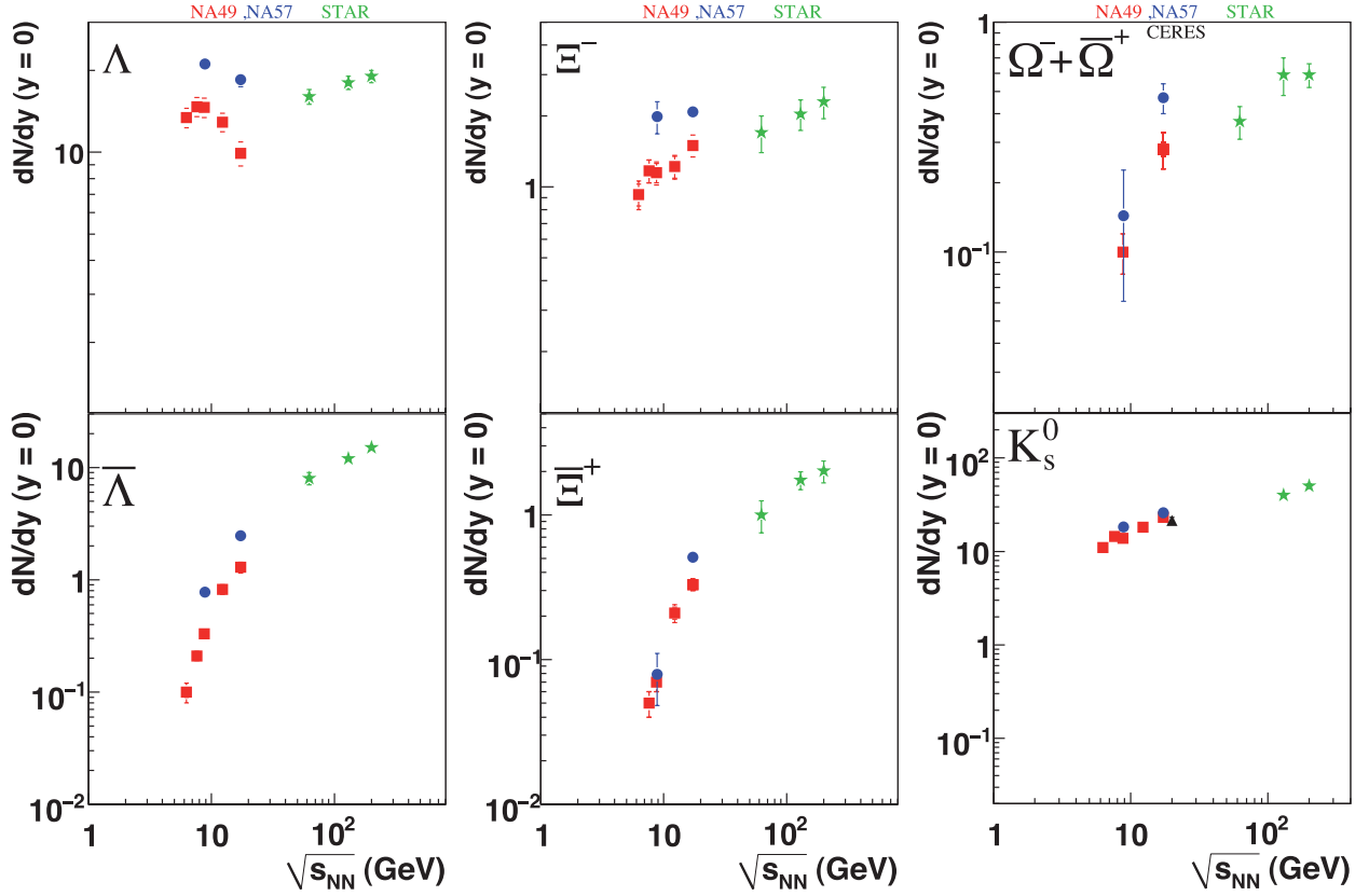
FIG. 51: The energy dependence of strange particle and anti-strange particle yields at midrapidity ( |y| \leq 0.5 ) from SPS to RHIC energies.
