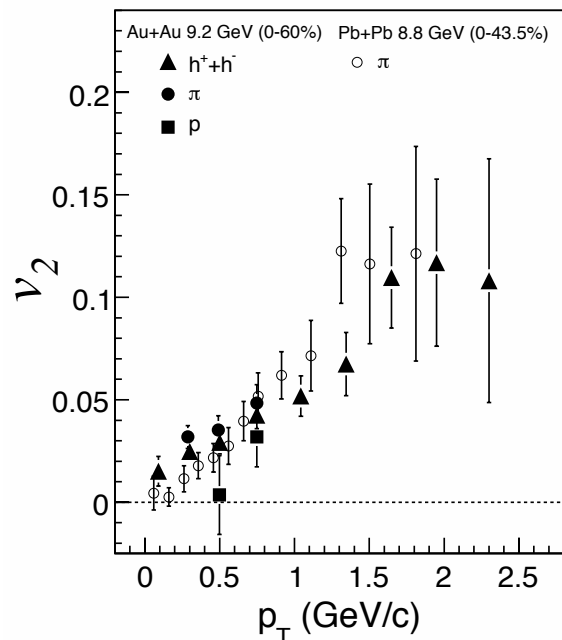
FIG. 59: The charged particle v_2 at \sqrt{s_{NN}} = 9.2 GeV as a function of p_T . From [105, 221].
