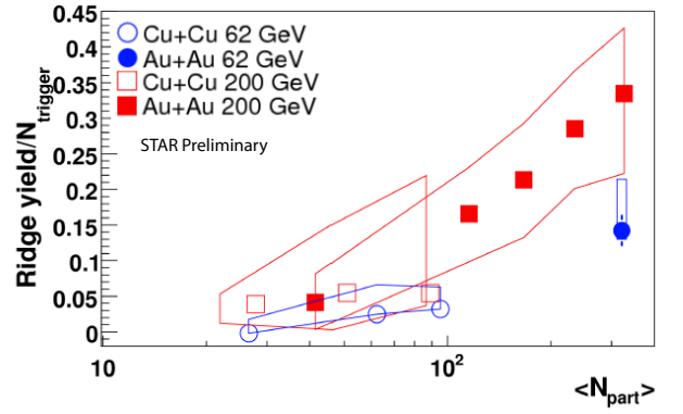
FIG. 47: The number of particles in the near side ridge correlation as a function of N_{\text{part}} for \sqrt{s_{NN}} = 200 and 62 GeV Cu+Cu and Au+Au collisions.
