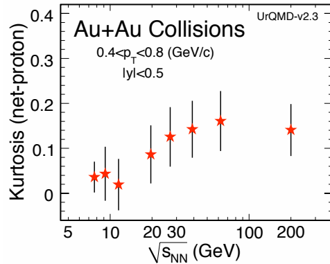
FIG. 17: The net-proton kurtosis from the UrQMD model, evaluated in the STAR acceptance for 100 k events.
