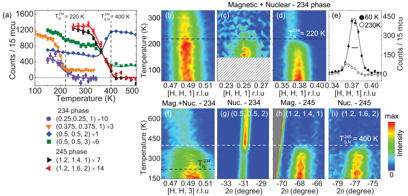
FIG. 2. (a) Temperature dependence of the peak intensities in \text{Rb}_{0.8}\text{Fe}_{1.5}\text{Se}_2 . The intensities for each peak have been normalized by a factor as shown following the corresponding wave vector. (b)–(f) The magnetic and superlattice peaks of the 234 phase scanned along the [H, H, 1] direction and (f) the [H, H, 3] direction. The bar in (e) indicates the instrumental resolution. (g) \theta - 2\theta scans of the rhombic iron vacancy order for the 234 phase at Q = (0.5, 0.5, 2) as a function of temperature. (h) \theta - 2\theta scans of the 245 phase through the magnetic peak Q = (1.2, 1.4, 1) and (i) the \sqrt{5} \times \sqrt{5} iron vacancy ordered peak Q = (1.2, 1.6, 2) . The black and white dashed lines mark the Néel temperature of the 234 phase at T_N^{234} = 220 K and the coincidental magnetic and structure transition temperature of the 245 phase at T_{s,N}^{245} = 400 K, respectively. The intensities in (b)–(i) have been normalized for better comparison. The lattice constants are chosen as the average of the two phases with a = b = 3.991 Å and c = 14.017 Å in the tetragonal notation optimized at 60 K. The “mcu” in units of intensity is a defined monitor count unit, which we defined as 1 \text{ mcu} \approx 1 \text{ s} .
