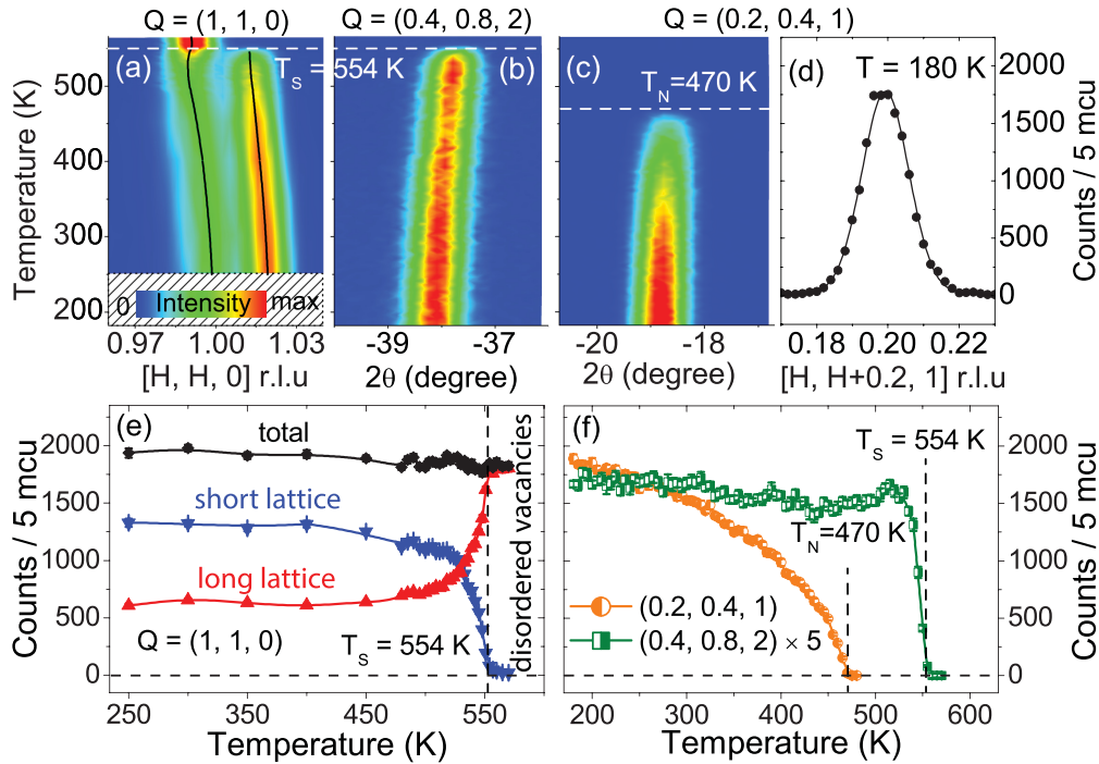
FIG. 4. Temperature dependence of neutron diffraction peaks in metallic \text{Rb}_{0.8}\text{Fe}_2\text{S}_2 . (a) Two well-separated peaks at Q = (1, 1, 0) along the [H, H, 0] direction. The left peak is associated with the 245 phase that has the lattice constants of a = b = 3.782 \text{ \AA} at 250 K, and the iron vacancy disordered phase with a = b = 3.811 \text{ \AA} at 570 K. The right peak belongs to the metallic phase with shorter lattice constants of a = b = 3.705 \text{ \AA} at 250 K. (b) \theta - 2\theta scans through the \sqrt{5} \times \sqrt{5} iron vacancy ordered peak at Q = (0.4, 0.8, 2) and (c) the block AF ordered peak at Q = (0.2, 0.4, 1) of the 245 phase. (d) A magnetic peak scan through Q = (0.2, 0.4, 1) along the [H, H + 0.2, 1] direction at 180 K. (e) The blue and red triangles are peak intensities extracted from the right and left peaks in (a), respectively. The peak widths are temperature independent. The black diamond is a sum of the two at each temperature. At temperatures above T_s = 554 \text{ K} , the two phases merge into an iron vacancy disordered phase. (f) Temperature dependence of the peak heights obtained from (b) and (c), respectively, which shows the Néel temperature at T_N = 470 \text{ K} and the iron vacancy order-disorder transition temperature at T_s = 554 \text{ K} . The intensities of the peak at Q = (0.4, 0.8, 2) have been multiplied by a factor of 5 in (b) and (f) for comparison.
