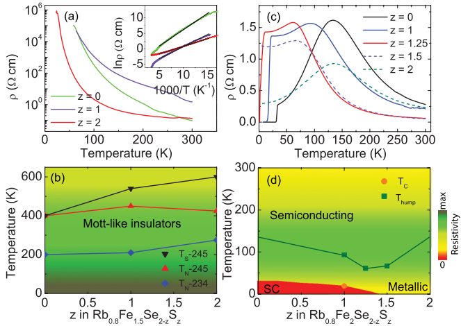
FIG. 5. (a) In-plane resistivity measurements of insulating \text{Rb}_{0.8}\text{Fe}_{1.5}\text{Se}_{2-z}\text{S}_z with z = 0, 1 , and 2 . The inset shows resistivity in logarithmic scale plotted against 1000/T , along with fits of \rho = \rho_0 \exp(E_a/k_B T) . (b) A phase diagram of insulating \text{Rb}_{0.8}\text{Fe}_{1.5}\text{Se}_{2-z}\text{S}_z as a function of sulfur doping. The solid lines mark the Néel temperatures of the 234 phase (blue), the 245 phase (red), and the \sqrt{5} \times \sqrt{5} iron vacancy order-disorder transition (black). (c) Resistivity measurements for \text{Rb}_{0.8}\text{Fe}_2\text{Se}_{2-z}\text{S}_z with z = 0, 1, 1.25, 1.5 , and 2 . (d) A phase diagram of \text{Rb}_{0.8}\text{Fe}_2\text{Se}_{2-z}\text{S}_z as a function of sulfur doping. The T_c 's and T_{\text{hump}} 's are extracted from (c). The color in (b) and (d) indicates the magnitude of resistivity.
