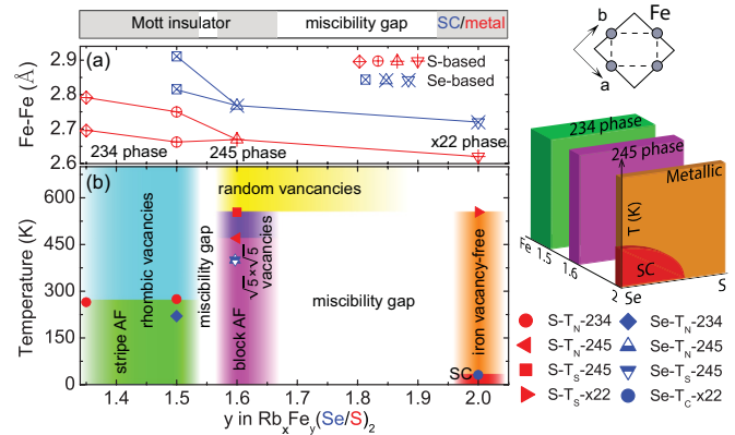
FIG. 6. (a) Fe-Fe bond lengths of the 234 phase, the 245 phase, and the “x22” phase for the S-based (red) and Se-based (blue) materials. The upper inset on the right is a sketch showing the Fe-Fe bonds along the two directions and the unit cell used throughout the paper marked by the solid line. (b) A phase diagram of temperature versus the iron content y in \text{Rb}_x\text{Fe}_y(\text{Se}/\text{S})_2 . The red and blue points are associated with the sulfide and selenide compounds, respectively. The white areas are miscibility gaps. The point at y = 1.35 is obtained from previous work [32]. The lower inset on the right is a schematic three-dimensional phase diagram with temperature, iron content, and Se:S ratio.
