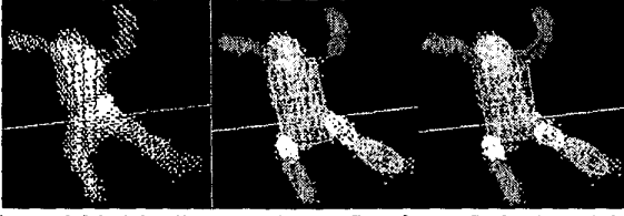
Figure 6 Model adjustment in the first frame. Left: the original voxel reconstruction. Middle: Body parts located in the initialization process. Note that the model is not valid at this stage – both arms are detached from the torso and right hip is at the side of the torso. Right: after the adjustment by the extended Kalman filter, the model is valid and fitted to the data.
