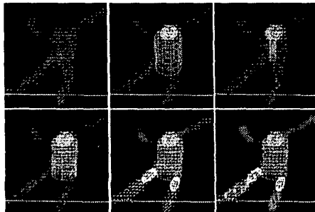
Figure 4 Model initialization. From left to right, top to bottom: (1) 3D silhouette, (2) head located and torso template after the initial positioning process, (3) shrunk torso template, (4) after the growing process, the torso voxels are labeled and the torso model fitted to them, (5) upper arms and thighs after the growing process, (6) lower arms and calves fitted onto the remaining voxels.
