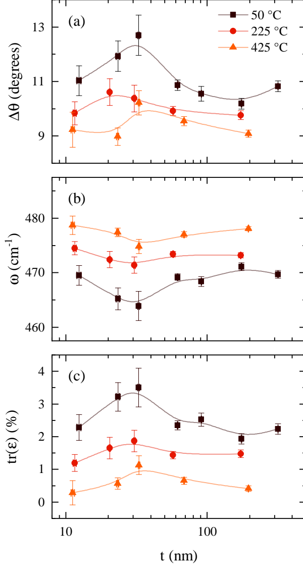
Figure 7. (a) Bond angle deviation \Delta\theta , (b) TO peak position \omega , and (c) trace of strain \text{tr}(\epsilon) as a function of thickness t for samples grown at 50 °C (brown squares), 225 °C (red circles) and 425 °C (orange triangles). Lines are guides to the eye.
