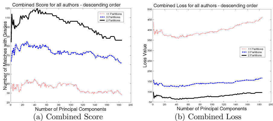
Fig. 11. Combined Score and Loss functions at all 3 partitions - Descending Order
