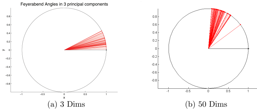
Fig. 4. Distance from Feyerabend to student essays as a function of dimension size
