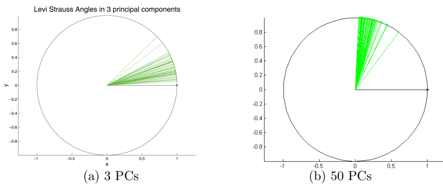
Fig. 5. Distance from Levi Strauss to student essays as a function of dimension size
