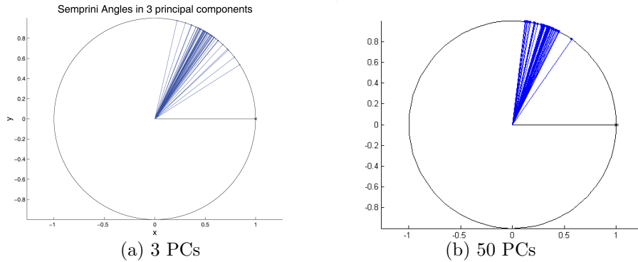
Fig. 6. Distance from Semprini to student essays as a function of dimension size
