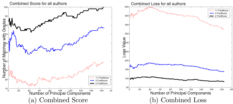
Fig. 10. Combined Score and Loss functions at all 3 partitions - Ascending Order
