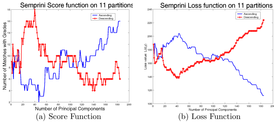
Fig. 8. Values of Score and Loss function for author Semprini with 11 partitions
