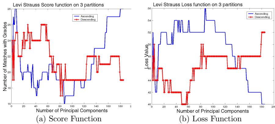
Fig. 9. Values of Score and Loss function for author Levi Strauss with 3 partitions
