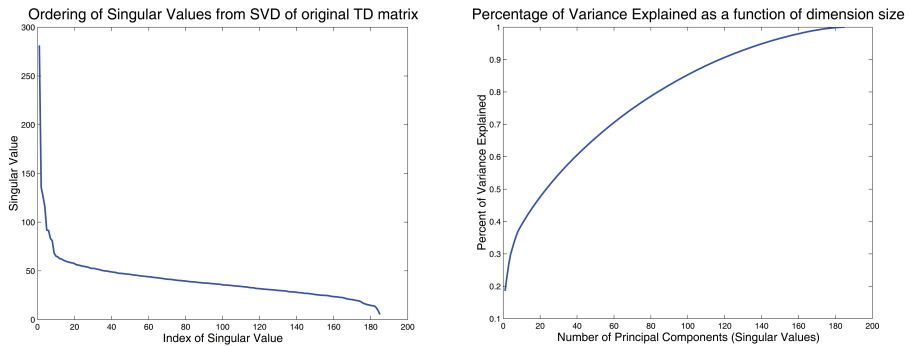
Fig. 3. Traditional Scree plot and Percent of Variance explained by first k principal components
