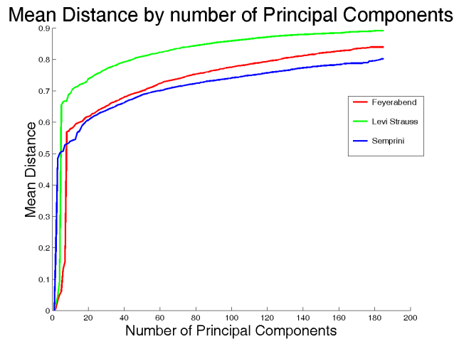
Fig. 7. Mean Distance from Author as a function of Principal Component
