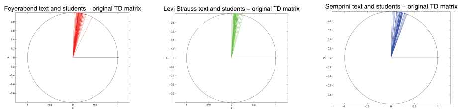
Fig. 2. Angular distance using original TD matrix
