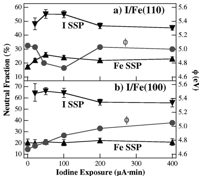
FIG. 1. Neutral fractions of ^7\text{Li}^+ singly scattered from the I and Fe sites, along with the surface work function ( \phi ) for I-adsorbed (a) Fe(110) and (b) Fe(100). The work function values for clean Fe(110) and Fe(100) were taken as 5.05 eV [26] and 4.67 eV [27], respectively.
