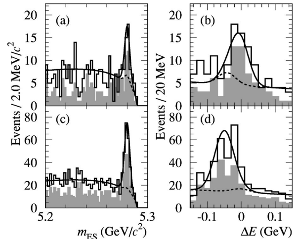
FIG. 1. Distributions of m_{ES} and \Delta E (unshaded histograms) for events enhanced in signal (a),(b) \pi\pi and (c),(d) K\pi decays based on the likelihood ratio selection described in the text. Solid curves represent projections of the maximum likelihood fit result after accounting for the efficiency of the additional selection, while dashed curves represent q\bar{q} and \pi\pi \leftrightarrow K\pi cross-feed background. Shaded histograms show the subset of events that are tagged.
