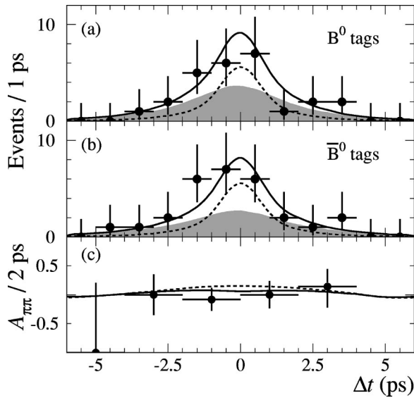
FIG. 2. Distribution of \Delta t for events enhanced in signal \pi\pi decays based on the likelihood ratio selection described in the text. (a) and (b) show events (points with errors) with B_{\text{tag}}=B^0 or \bar{B}^0 . Solid curves represent projections of the maximum likelihood fit, dashed curves represent the sum of q\bar{q} and K\pi background events, and the shaded region represents the contribution from signal \pi\pi events. (c) shows \mathcal{A}_{\pi\pi}(\Delta t) for data (points with errors), as well as fit projections for signal and background events (solid curve), and signal events only (dashed curve).
