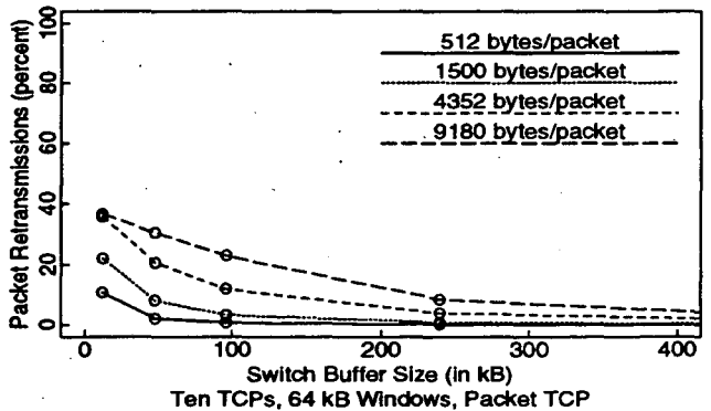
Figure 10: Packet Retransmission Rates for Packet TCP
