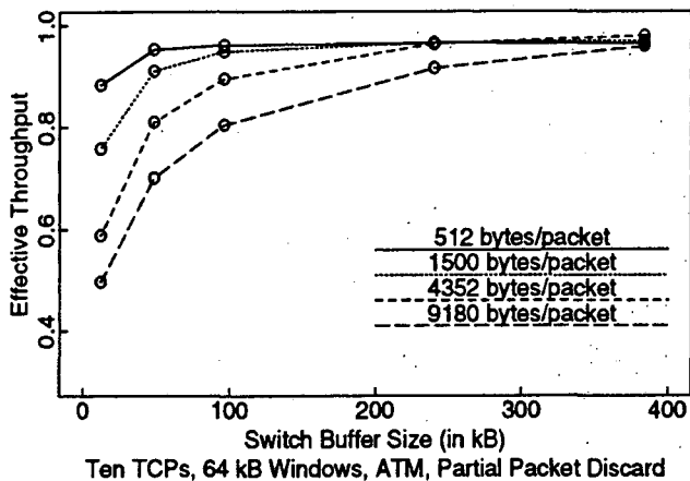
Figure 4: Partial Packet Discard
