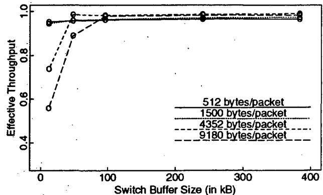
Figure 5: Early Packet Discard
