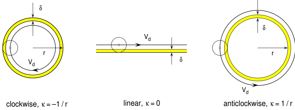
Figure 1: Estimation of the chip load in machining a depth of cut \delta with a tool of radius d moving with feedrate V_d for (left) an interior cut on a circle of radius r ; (center) a linear cut; and (right) an exterior cut on a circle of radius r . The shaded areas identify the material strip removed from the workpiece.
