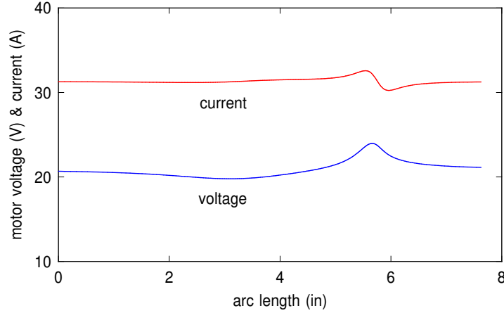
Figure 6: Variation of the motor voltage \mathcal{V} and current I to achieve a constant chip load c , for a fixed feedrate and depth of cut along the path in Figure 2. The motor specifications and other parameters are as prescribed in the text.
