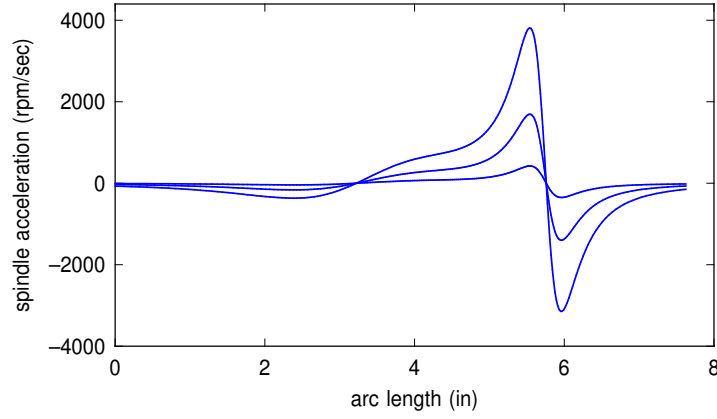
Figure 5: The spindle angular acceleration (24) for a depth of cut \delta = 0.05 in along the curve in Figure 2, using a tool with radius d = 0.25 in and m = 3 flutes, for a constant chip load c = 0.005 in and feedrates V_d = 20 in/min, 40 in/min, and 60 in/min along the offset path — the increasing amplitudes of the angular acceleration correspond to the increasing feedrate values.
