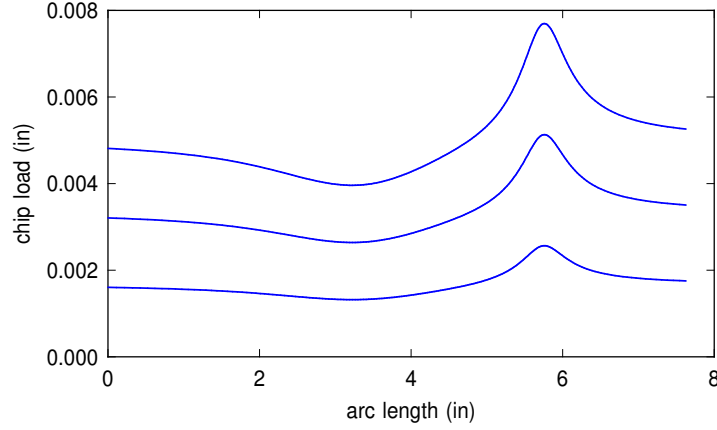
Figure 3: Variation of the chip load (19) for a depth of cut \delta = 0.05 in along the curve in Figure 2, using a tool with radius d = 0.25 in and m = 3 flutes at constant spindle speed n = 4000 rpm, and constant feedrates V_d = 20 in/min (lower), 40 in/min (middle), and 60 in/min (upper) along the offset path.
