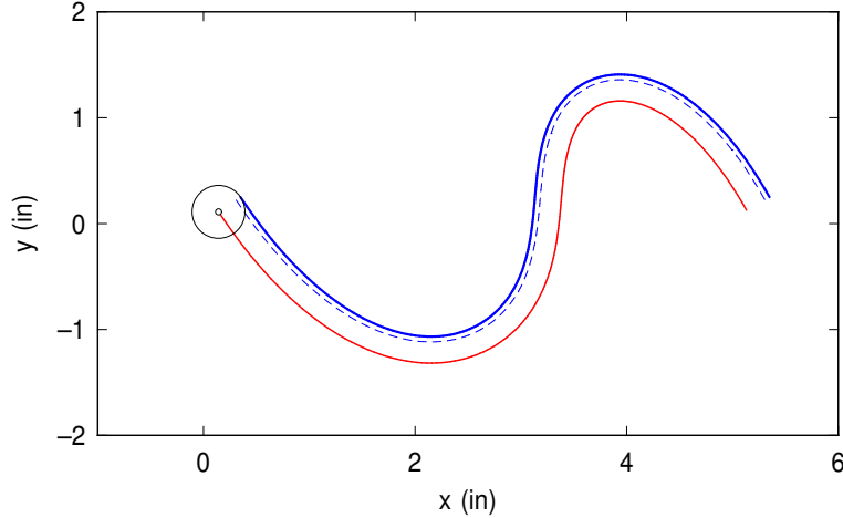
Figure 2: The desired part shape \mathbf{r}(\xi) is indicated by the blue curve, while the dashed blue curve indicates the depth of cut \delta = 0.05 in to be removed. The red curve indicates the offset path (7) for a tool of radius d = 0.25 in.
