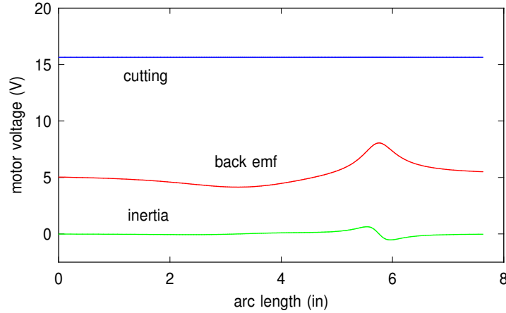
Figure 7: The three terms in (31) that determine the motor voltage \mathcal{V} — the back emf term k\omega , cutting term RfP/k\omega , and inertia term (RJ/k) d\omega/dt .
