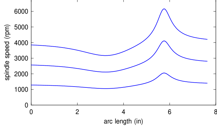
Figure 4: Variation of the angular velocity (20) for a depth of cut \delta = 0.05 in along the curve in Figure 2, using a tool with radius d = 0.25 in and m = 3 flutes, for a constant chip load c = 0.005 in and feedrates V_d = 20 in/min (lower), 40 in/min (middle), and 60 in/min (upper) along the offset path.
