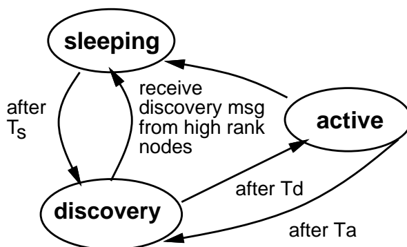
Figure 3: State transitions in GAF.
