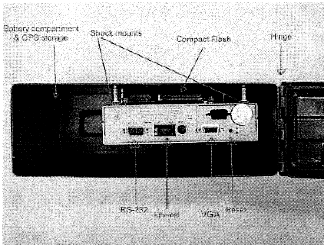
Figure 2: Extensible data collection unit, interior, showing the hardware layout and the different data ports.
