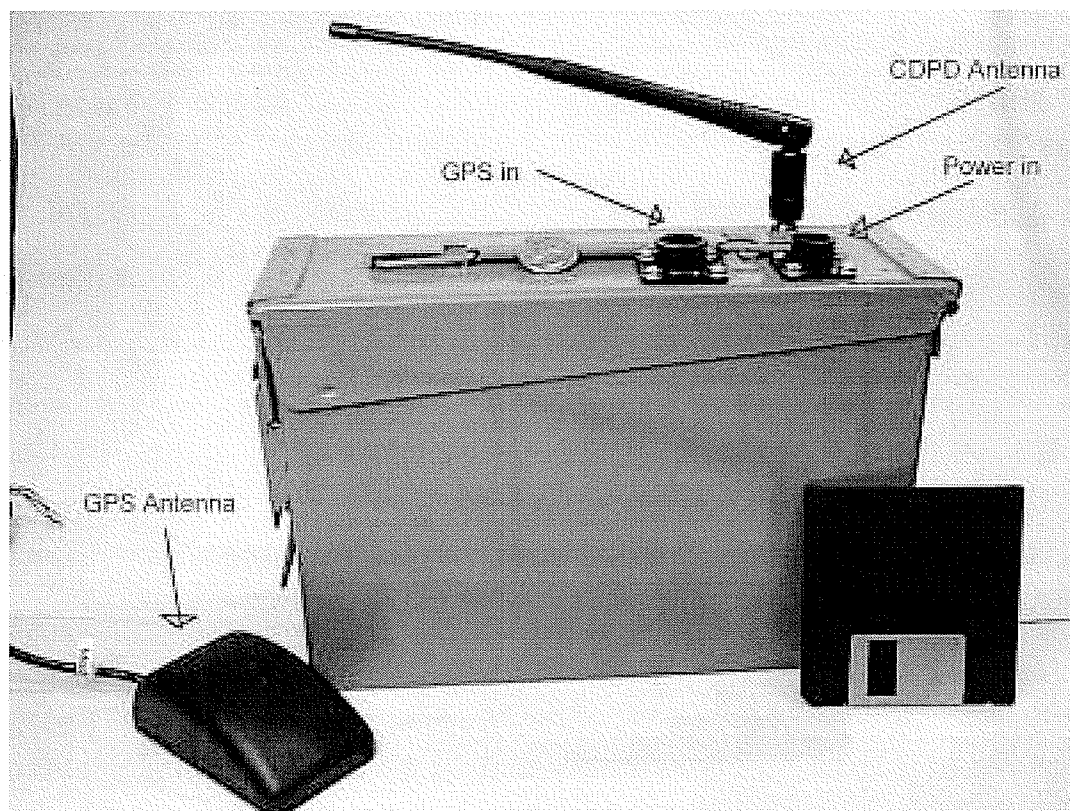
Figure 1: Extensible data collection unit, complete with GPS antenna and cellular data modem antenna.
