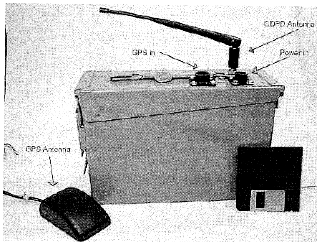
Figure 1: Extensible data collection unit, complete with GPS antenna and cellular data modem antenna.
