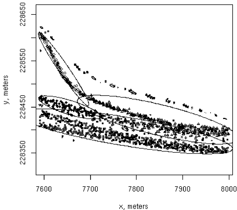
Figure 18. Agglomerative Clustering of Figure 16 Data Points
