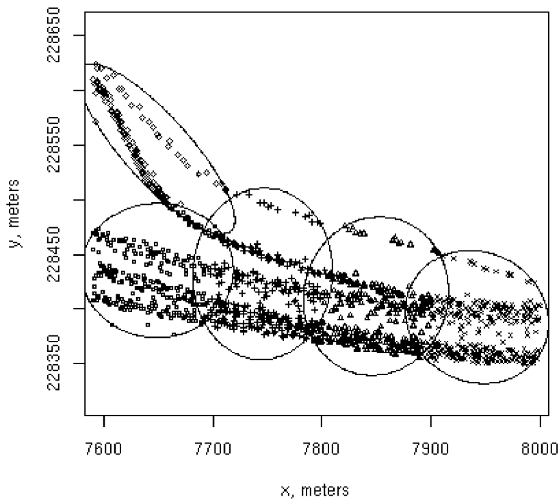
Figure 17. K-means clustering of Figure 16 Data Points
