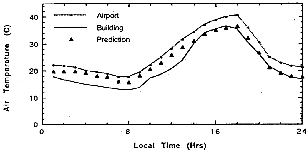
Figure 1: Diurnal air temperature profiles measured at a residential site and the nearby airport. Symbols represent Method 1 prediction of the residential site diurnal temperature profile.
