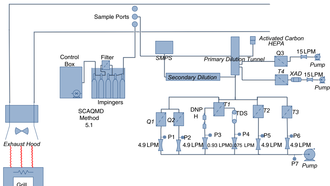
Fig. 1 – Schematic of sampling system for measurement of particle phase and gas phase compounds. SMPS: Scanning Mobility Particle Spectrometer; DNP H: Dinitrophenylhydrazine; XAD: Polyaromatic absorbent resin; LPM: liters per minute; TDS: thermal desorption tubes; Q1: quartz filter #1; Q2: quartz filter #2; Q3: quartz filter #3; T1: teflon filter #1; T2: teflon filter #2; T3: teflon filter #3; T4: teflon filter #4; P1: pressure 1; P2: pressure 2; P3: pressure 3; P4: pressure 4; P5: pressure 5; P6: pressure 6; P7: pressure 7; HEPA: high-efficiency particulate arrestance.
