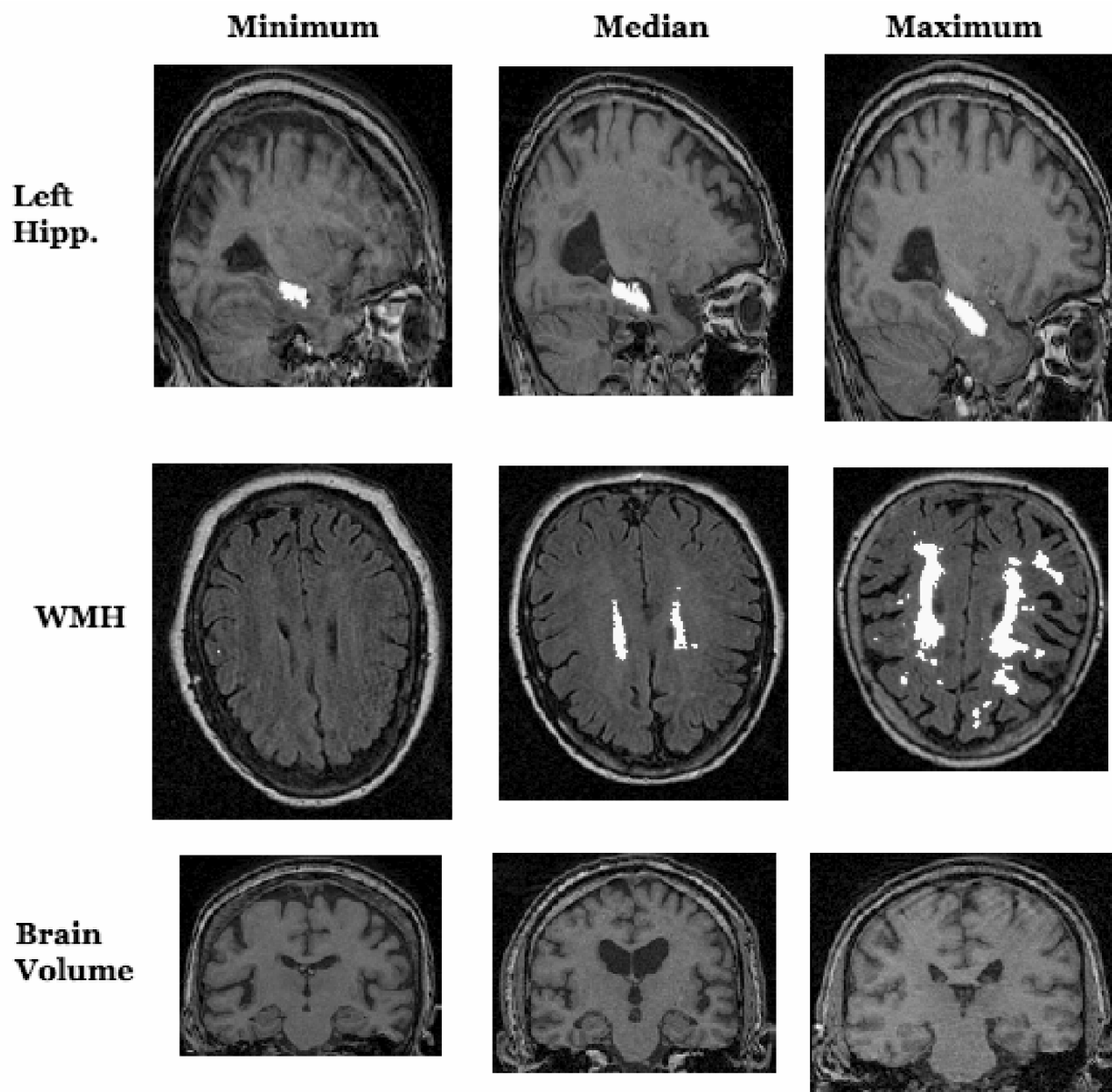
Figure 3: Characteristic slices from MRI scans of individuals who had the minimum, median, and maximum values of left hippocampal volume, WMH volume, and brain volume. The left hippocampus is annotated by a white overlay on sagittal slices of T1-weighted images, and WMHs are annotated by a white overlay on axial slices of FLAIR images. Note that in the statistical analysis, brain and hippocampal volume were adjusted to account for inter-individual differences in intracranial volume.
