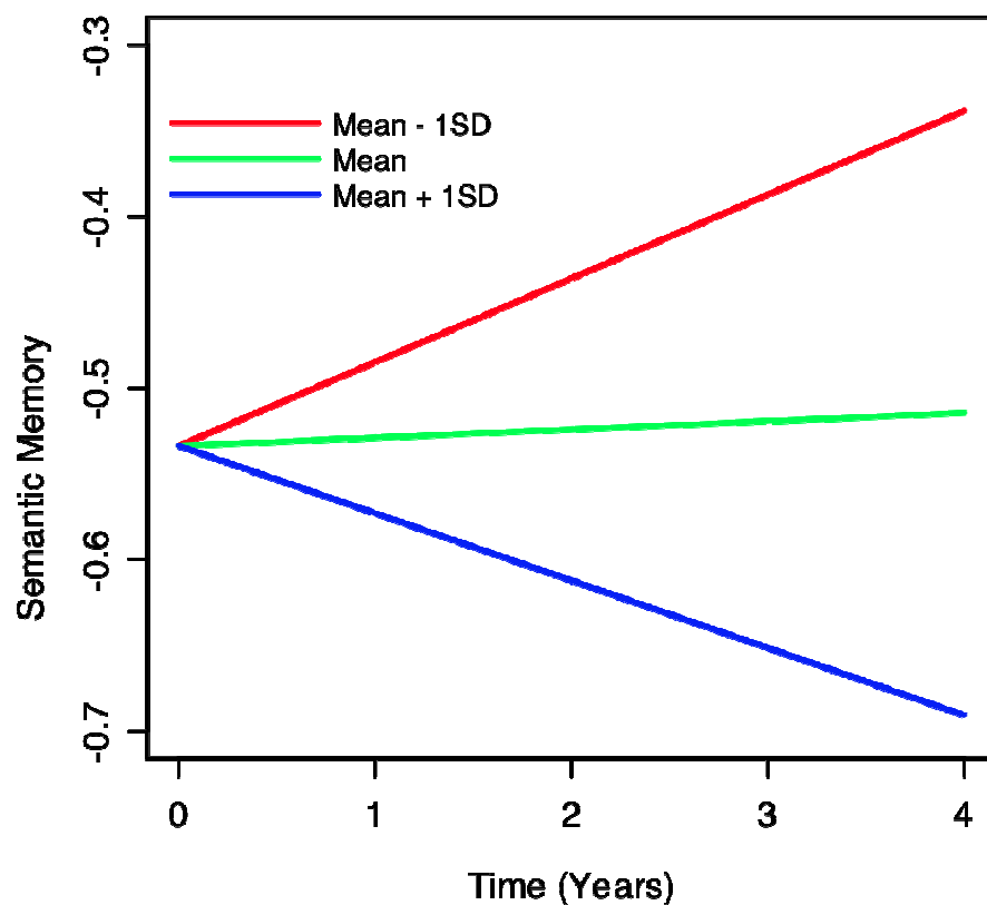
Figure 2: Example longitudinal trajectories of executive function and semantic memory, and the effect of WMH volume in modifying those trajectories. Each line represents the estimated cognitive trajectory for a hispanic female with mean educational attainment (12.6 years), mean BV (919.1 cm 3 ), and mean HC (3.62 cm 3 ). The three lines per plot represent the estimated trajectories of an individual that exhibits these characteristics along with differing levels of BV: the population mean, the mean plus one standard deviation, and the mean minus one standard deviation. The executive function and semantic memory scores are scaled as z-scores; the mean of these measures over the entire population is 0 and a one-unit difference represents a difference of one standard deviation.
