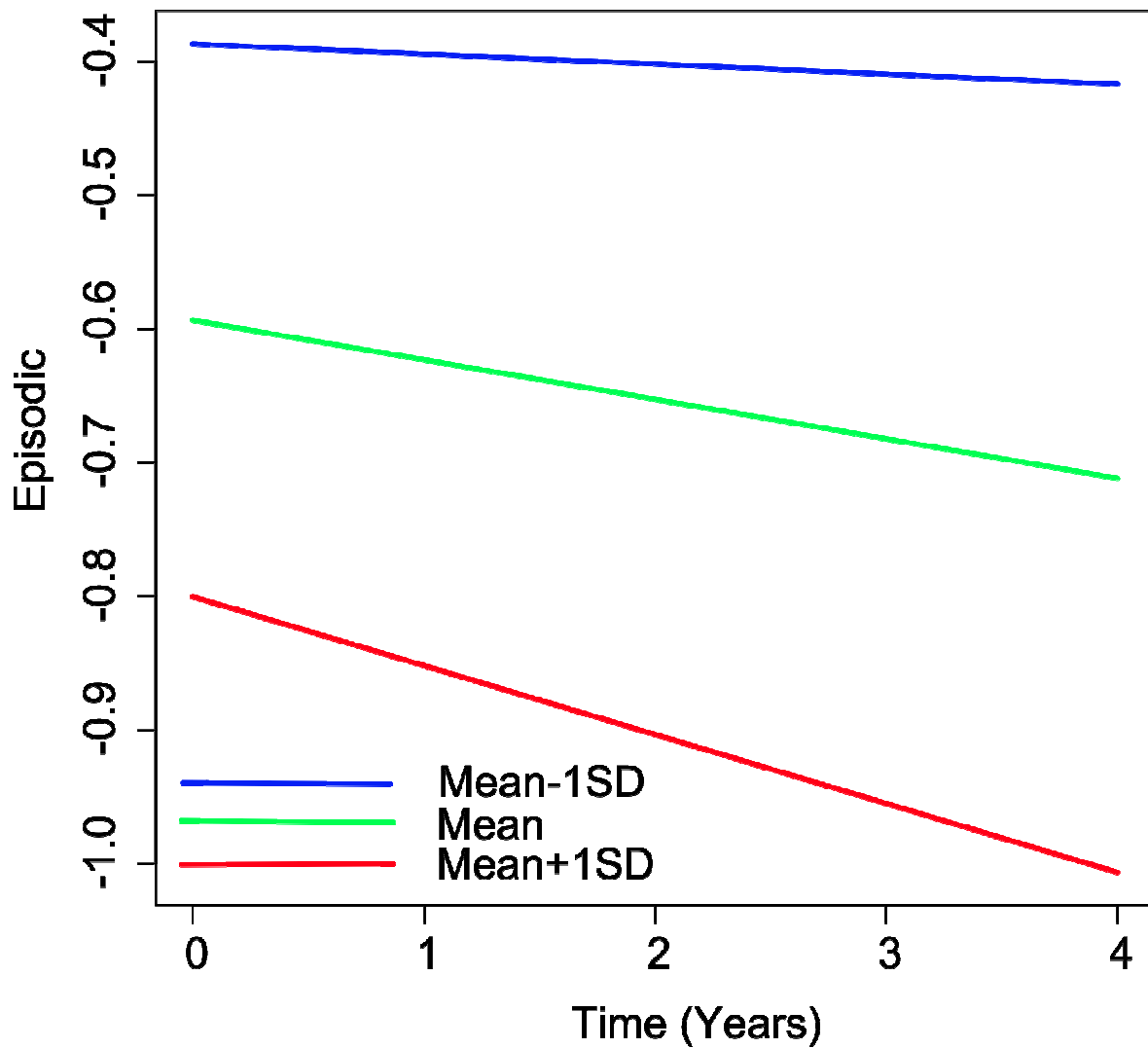
Figure 1: Example longitudinal trajectory of episodic memory, and the effect of brain volume in modifying that trajectory. Each line represents the estimated cognitive trajectory for a Hispanic female with mean educational attainment (12.6 years), mean WMH (9.10 cm 3 ), and mean HC (3.62 cm 3 ). The three lines per plot represent the
