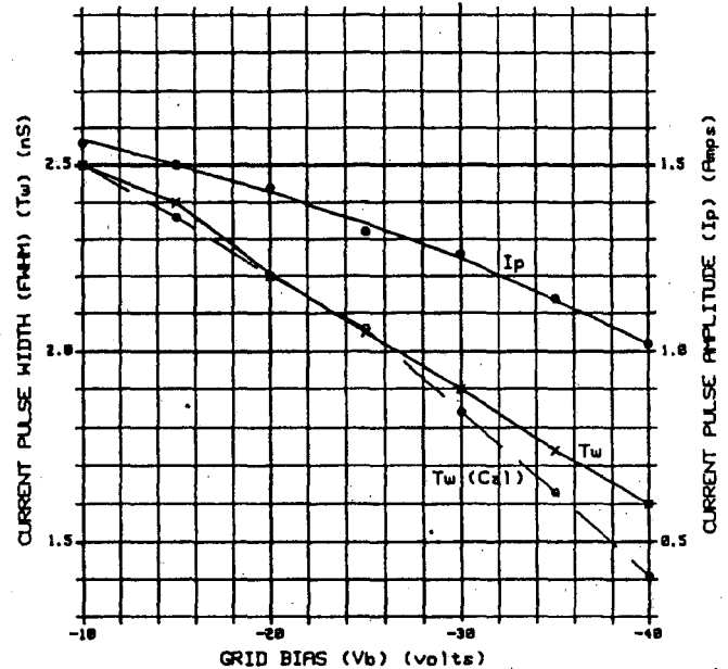
Figure 2. Current pulse width and amplitude vs grid bias.
