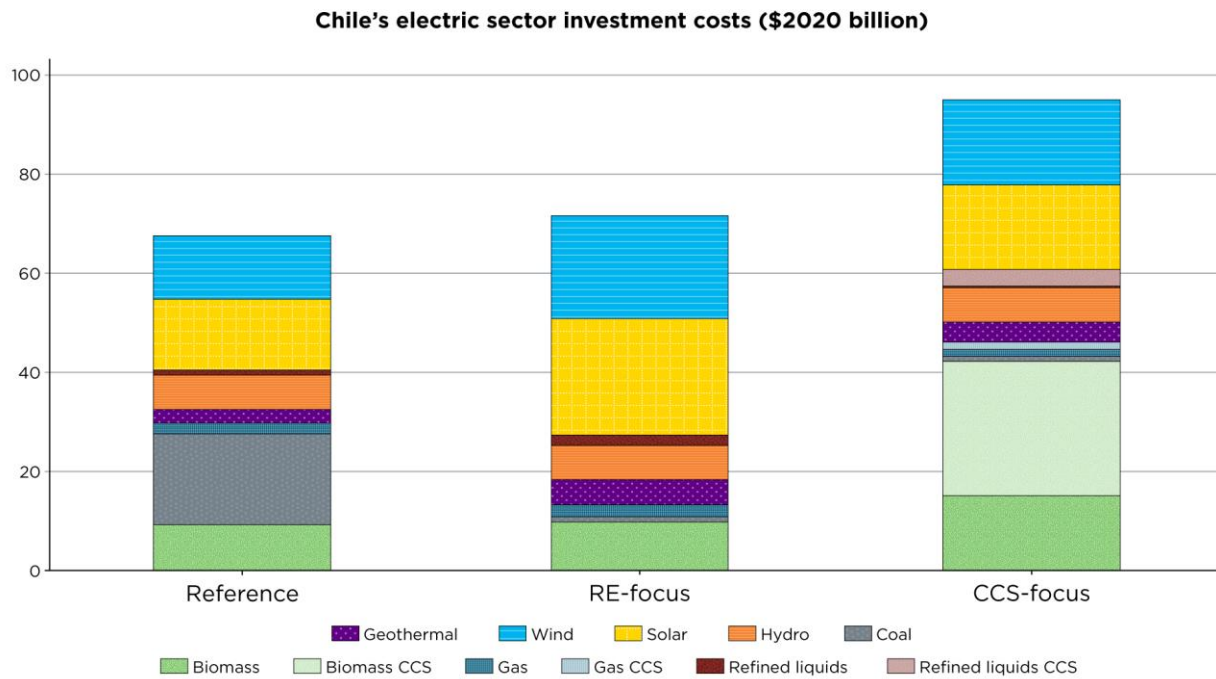
Figure 28. Chile's electric sector investment costs, 2020–2050
