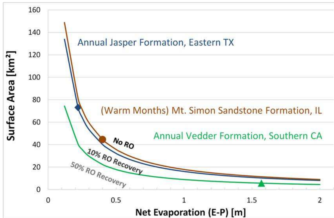
Figure S1: Surface area of evaporation ponds as a function of average net evaporation (evaporation E – precipitation P) rates and reverse osmosis (RO) freshwater recovery fraction. Solid symbols show the SA required to hold the brine from one carbon dioxide capture and sequestration (CCS) project in three saline aquifers: Mt. Simon (orange circle), Vedder (green triangle), and Jasper (blue diamond).
