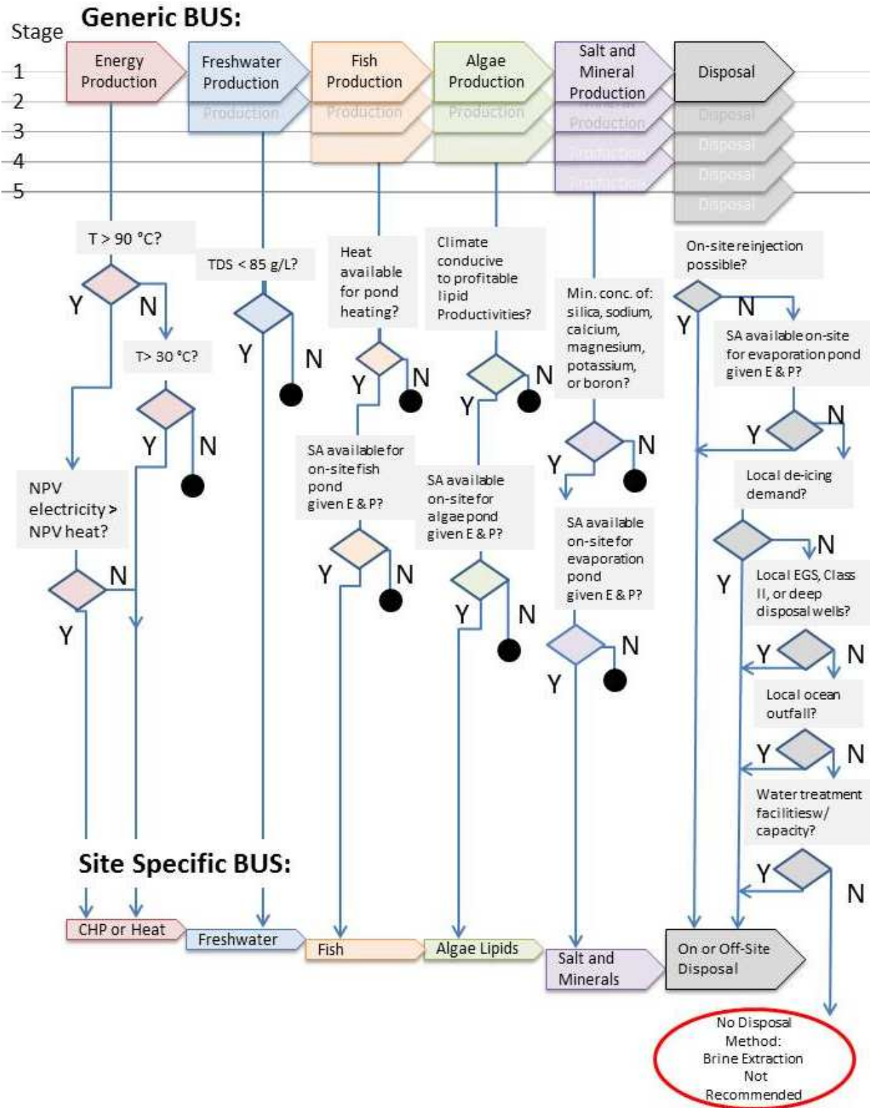
Figure 2: System Diagram. This diagram shows on- and off-site resource harvesting, treatment and disposal stages included in the study. Inputs include parameters like brine temperature (T), brine TDS, treatment net present value (NPV) and surface area (SA) requirements calculated from evaporation (E) or precipitation (P) data. Combined heat and power (CHP) is the generation of electricity as well as heat.
