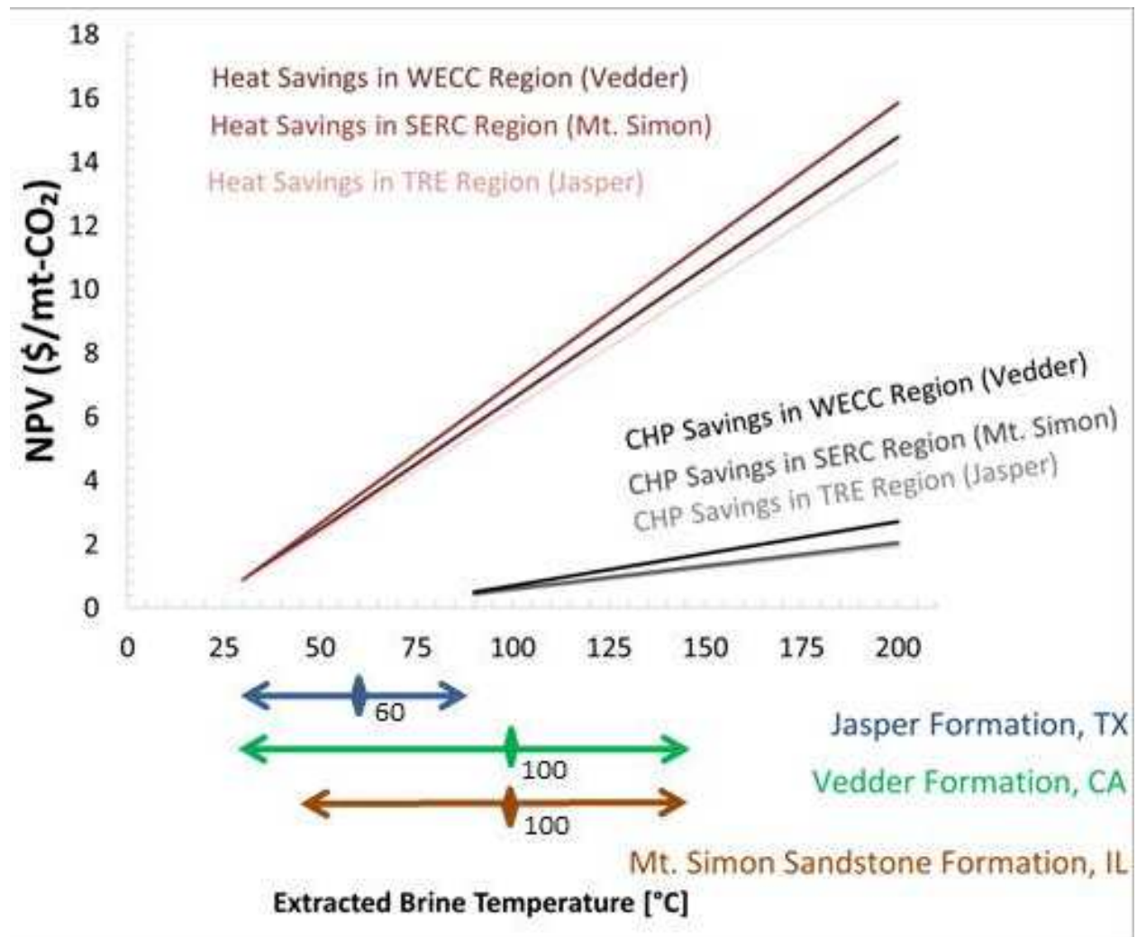
Figure 4: Parameter variation analysis for energy production. Geothermal energy can be used for (1) heating aquaculture ponds if brine T is above 30 °C, and (2) combined heat and power (CHP) if brine T is above 90 °C. Temperature ranges for saline aquifers are shown as solid arrows below graph. Representative aquifer temperatures are marked as diamonds on the solid arrows.
