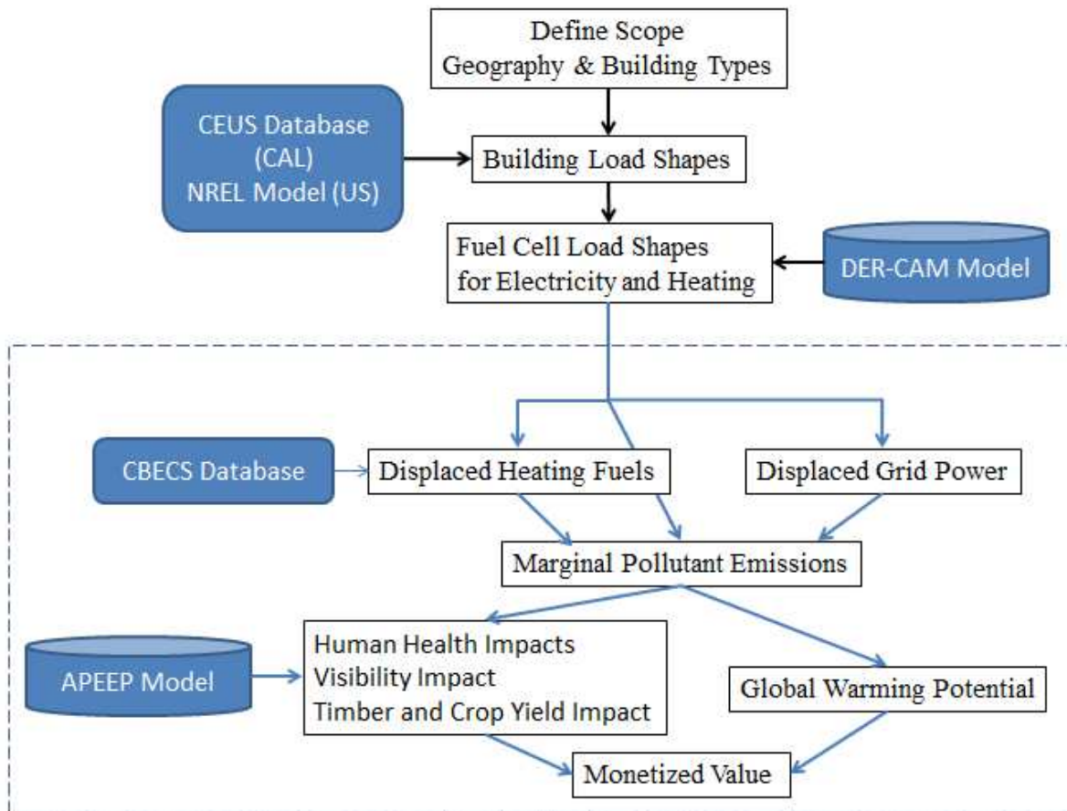
Figure A4. Flow diagram showing how steps in the model presented in this dissertation (dashed box) supports the model developed in Wei et al. External databases and models are shown. New acronyms: California Commercial End-Use Survey (CEUS); National Renewable Energy Laboratory (NREL); Distributed Energy Resources Customer Adoption Model (DER-CAM).
