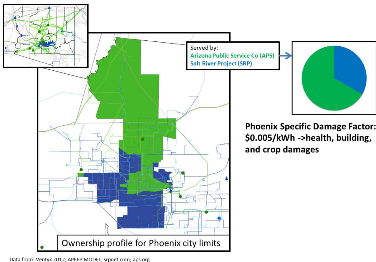
Figure A1. Power Service Area for Phoenix Arizona. Lines represent distribution and transmission lines, with blue representing capital owned by the Salt River Project and green representing capital owned by the Arizona Public Service Co. Points represent power generators (sun icons represent solar farms and drops represent hydroelectric generators). The inset shows the geospatial footprint of the two company's capital. For example, the Four Corners is the coal fired power plant in New Mexico in the upper right-hand corner of the inset. Data was gathered from Ventyx 2012, srpnet.com, and aps.com. Tear-drops indicate hydro-power and circles indicate solar power. Pie chart shows percent of annual generation provided by each company.
