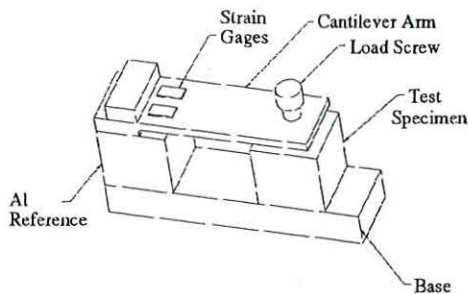
Fig. 2. Sketch of differential thermal contraction measurement fixture.
