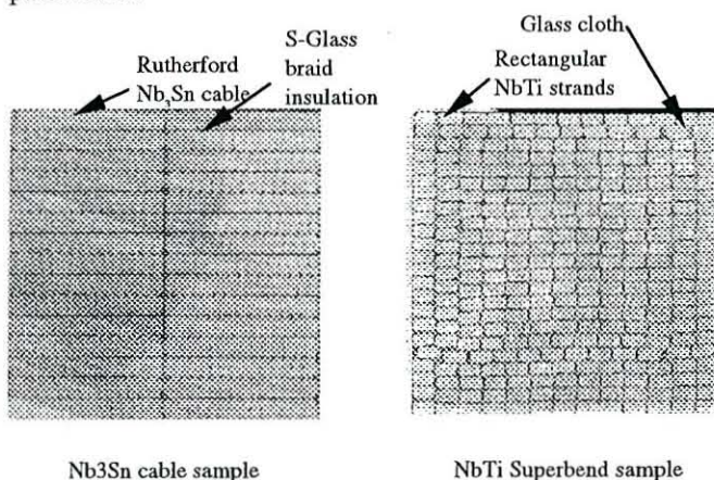
Fig. 1. Image of sample cross sections. Horizontal and vertical directions correspond to axial and radial directions, respectively. Tangential direction is normal to page.
