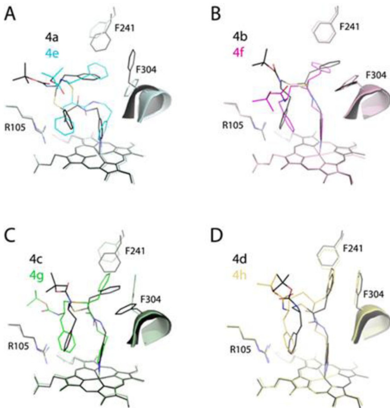
Figure 7. Pairwise comparison of the 4a-4e (A), 4b-4f (B), 4c-4g (C) and 4d-h (D) pairs showing that stereochemical restraints and the pyridyl-linker extension are compensated through changes in the backbone curvature and reorientation of the R 1 -phenyl, Phe241 and Phe304 rings.
