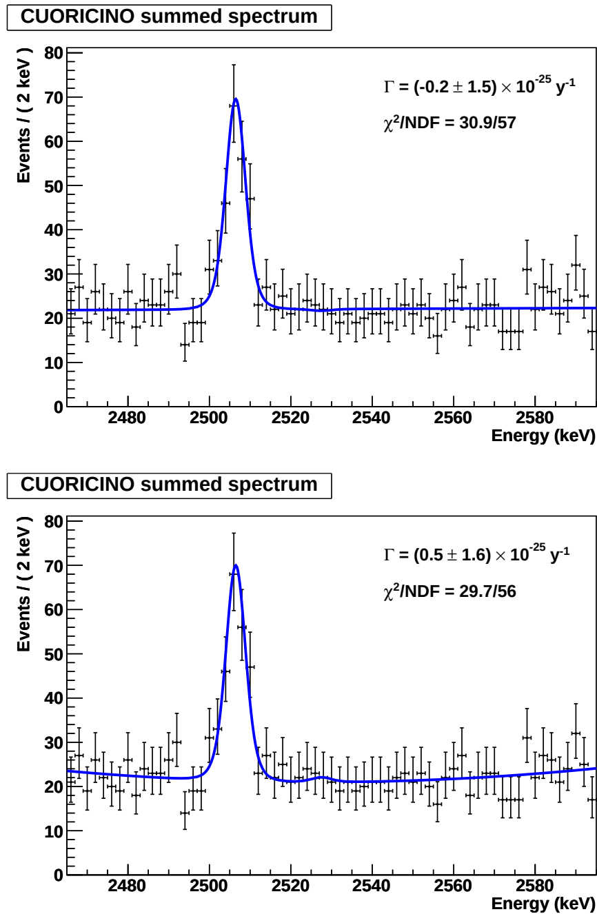
Figure 6.11: Fit projected onto the summed spectrum with a first order polynomial background (top) and a second order polynomial background (bottom). The \chi^2 and number of degrees of freedom (NDF) for these graphs are displayed to provide a measure of the goodness-of-fit, although this \chi^2 is not the quantity that is minimized to determine the fit parameters.
