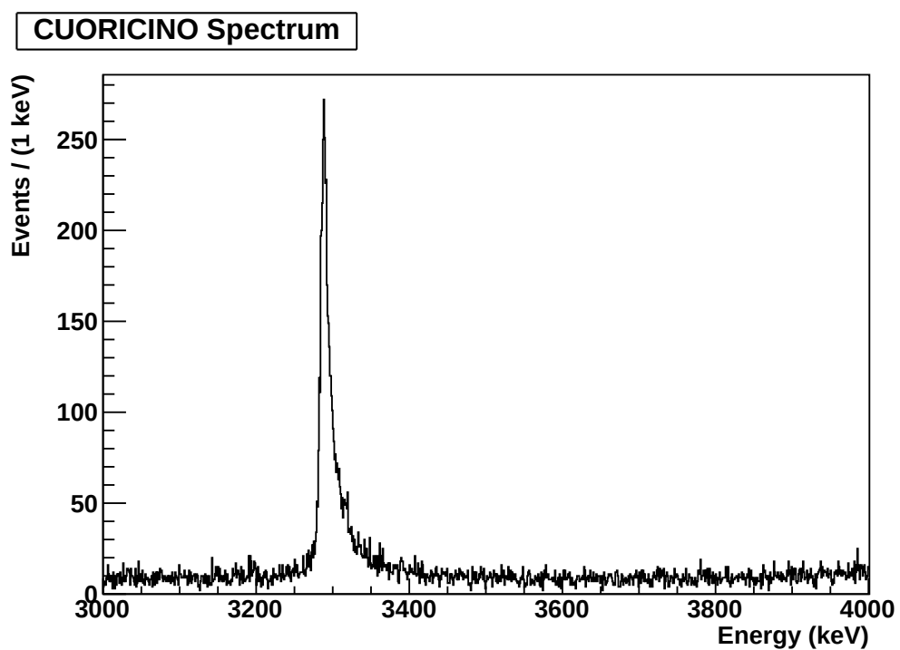
Figure A.2: CUORICINO spectrum calibrated with a third-order polynomial function below 3000 keV and calibrated with a second-order log polynomial function above 3000 keV.
