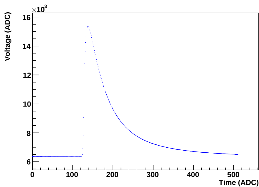
Figure C.1: A CUORICINO pulse on channel 7 of run 737. This pulse was caused by a gamma from the 2615 keV line of ^{208}\text{Tl} . The units on the vertical axis are ADC values, and the units on the horizontal axis are digital samples.
