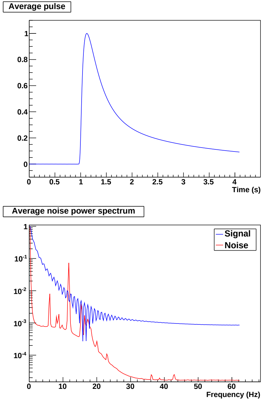
Figure 4.2: Top: The average pulse for CUORICINO channel 1. Bottom: The average noise power spectrum (red) and the modulus of the discrete Fourier transform of the average pulse (blue) for CUORICINO channel 1 (scaled to be equal at the lowest frequency).
