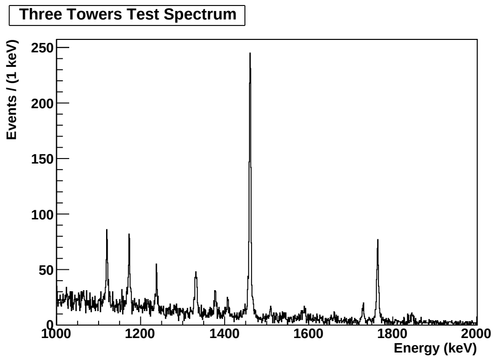
Figure A.5: Three Towers Test spectrum without ^{40}\text{K} sources.
