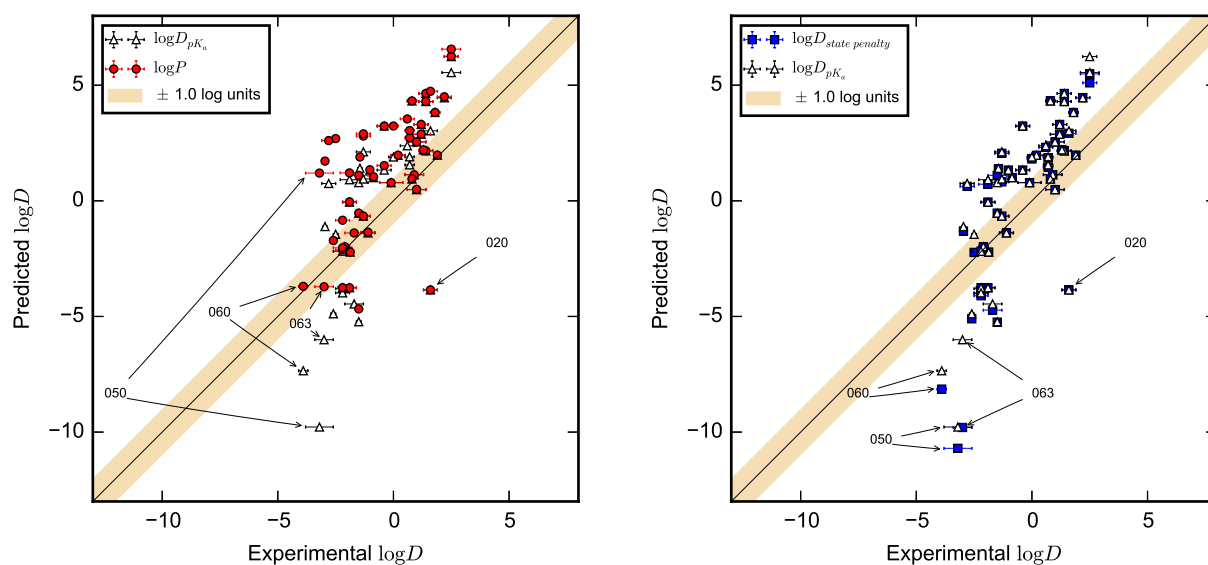
Fig. 7 Plots showing our reference calculations compared to experiment. Shown here is the results for submission 39 in SAMPL5, with no tautomer correction ( \log P ), distribution coefficient corrected from calculated partition coefficient based on pKas ( \log D_{pK_a} ), and distribution coefficient corrected from calculated partition coefficient based on state penalties ( \log D_{state\ penalty} ).
