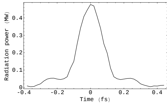
Figure 8: Estimated attosecond pulse power at 4-nm wavelength from a radiator with N_R = 25 .
