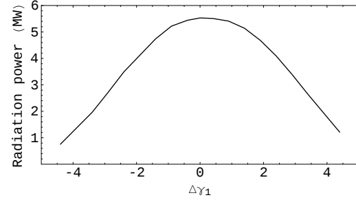
Figure 4: Predicted peak radiated power versus detuning from the FEL resonance energy in the UM.
