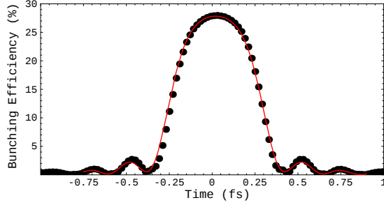
Figure 2: Bunching efficiency at 1-nm wavelength versus time along the electron bunch. The solid line shows analytical prediction and the dots simulation results from GINGER. The FWHM of the peak is 530 attoseconds.
