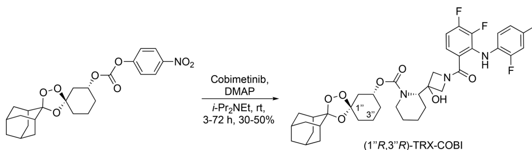
Scheme 1. (1''R, 3''R)-dispiro[adamantane-2,3'-[1,2,4] trioxolane-5',1''-cyclohexan]-3''-yl (S)-2-(1-(3,4-difluoro-2-((2-fluoro-4-iodophenyl)amino)benzoyl)-3-hydroxyazetidino-3-yl)piperidine-1-carboxylate.
