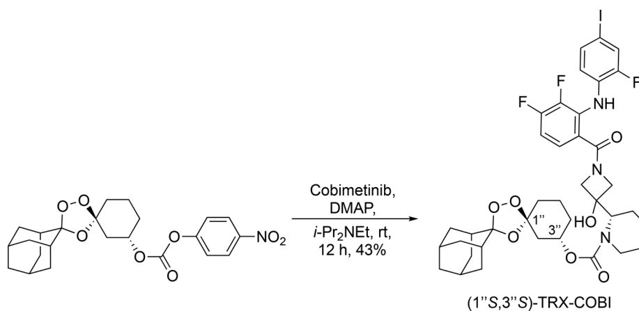
Scheme 2. (1''S,3''S)-dispiro[adamantane-2,3'-[1,2,4]trioxolane-5',1''-cyclohexan]-3''-yl(S)-2-(1-(3,4-difluoro-2-((2-fluoro-4-iodophenyl)amino)benzoyl)-3-hydroxyazetidino-3-yl)piperidine-1-carboxylate.
