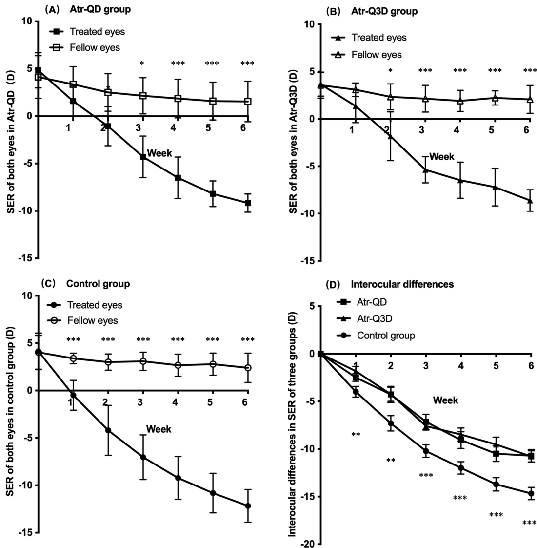
Figure 1. SERs (Mean \pm SEM) plotted against time for guinea pigs wearing a negative contact lens on their right eyes for 6 weeks ( -10 D, 0-3 weeks, -15 D, 3-6 weeks), with the same eyes treated with topical 1% atropine daily (Atr-QD) (A), or every 3 days (Atr-Q3D) (B), or with artificial tears daily (control) (C); interocular differences in SERs (mean \pm SEM), recorded for the same 3 groups and time intervals shown in (D). * P < 0.05 ; ** P < 0.01 ; *** P < 0.001 .
