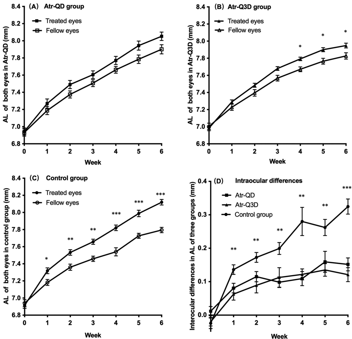
Figure 2. ALs (mean \pm SEM) plotted against time for guinea pigs wearing a negative contact lens on their right eyes for 6 weeks ( -10 D, 0 – 3 weeks, -15 D, 3 – 6 weeks), with the same eyes treated with topical 1% atropine daily (Atr-QD) (A), or every 3 days (Atr-Q3D) (B), or with artificial tears daily (control) (C); interocular differences in ALs (mean \pm SEM), recorded for the same 3 group and time intervals shown in (D). * P < 0.05 ; ** P < 0.01 ; *** P < 0.001 .
