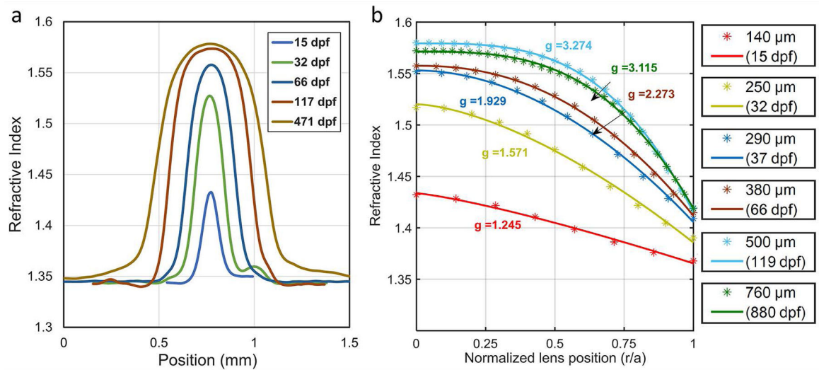
Figure 5. Fits of normalised GRIN profile to the exponential power model
