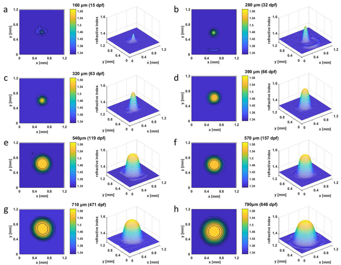
Figure 4. 2D and 3D refractive index distribution plots
