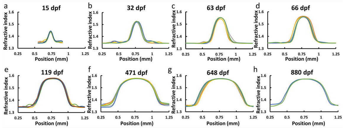
Figure 7. GRIN profiles with age
