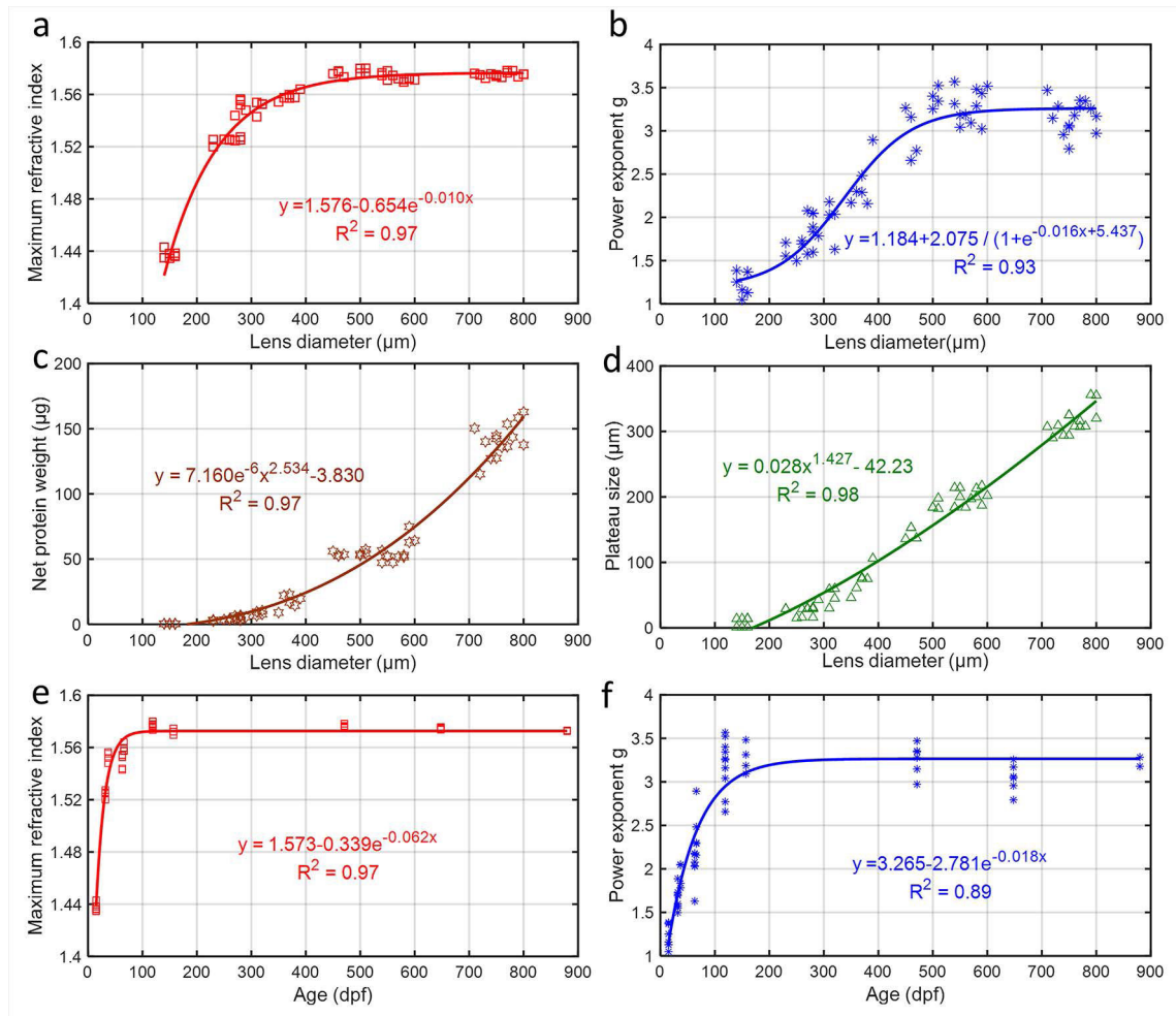
Figure 6. Growth of GRIN profile parameters and lens net protein weight with development (a) Maximum refractive index value plotted against lens diameter, (b) fitted power exponent g plotted against lens diameter, (c) net protein weight plotted against lens diameter, (d) size of central plateau region of each lens plotted against lens diameter, (e) maximum refractive index value plotted against age in dpf and (f) fitted power exponent g plotted versus age in dpf.
