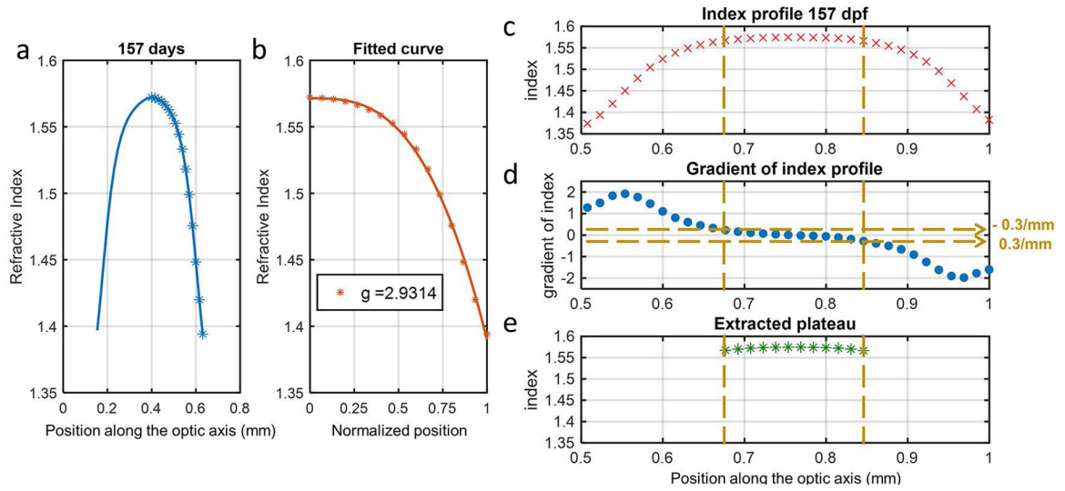
Figure 2. Parameters characterizing gradient refractive index (GRIN) profiles of zebrafish lenses (a) GRIN profile plotted against position along the optic axis for a 157 day old lens and (b) GRIN profile of the same lens normalised to the half length of the optic axis and points showing fits to the power exponent model with the value of the power exponent g for the best fit given (c) full GRIN profile of a 157 day old lens, (d) first order derivative of GRIN profile at 157dpf to show over which parts of the profile it shows a plateau and (e) determined plateau region of the GRIN profile.
