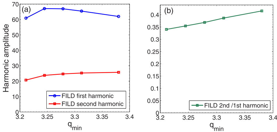
FIG. 16. (a) The first and second harmonic amplitude and (b) the ratio of the second harmonic over the first harmonic VS q value. The n=2 mode structures and frequencies for different q values are shown in Fig. 12, where the amplitude given here is B_{\max}/B_0 = 0.002 .
