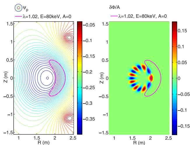
FIG. 1. Poloidal magnetic flux of DIII-D pulse 146 096 at 365 ms, given the perturbed AE electrostatic field normalized by the amplitude, and the equilibrium test particle orbit, where \lambda = \mu B_0 / E is the test particle’s pitch angle. Only the inner leg of the banana orbit can interact with the localized AE mode.
