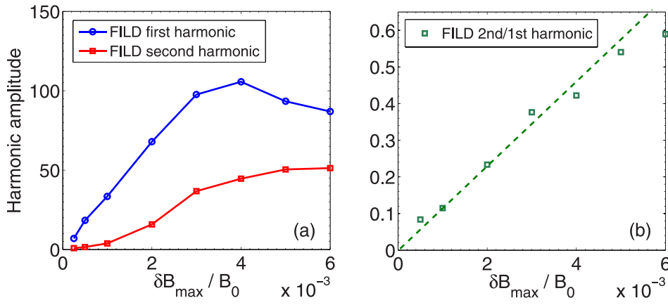
FIG. 15. FILD spectrum: (a) first and second harmonic amplitudes VS wave amplitude and (b) the ratio of the second harmonic over the first harmonic VS wave amplitude for AE modes shown in Fig. 13(a), q_{\min} = 3.28 and n = 3 cases.
