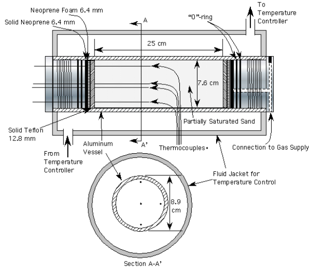
Figure 1. Vessel schematic.
