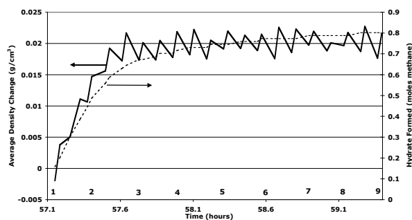
Figure 7. Average change in density (heavy line) and moles of methane converted to hydrate (dashed line) during the second hydrate formation. Numbers correspond to images in Figure 6.
