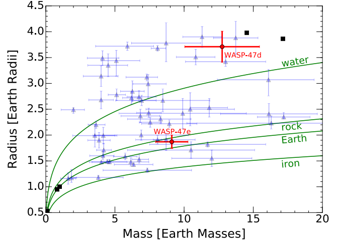
FIG. 2.— Radii and masses of all confirmed planets whose mass and radius are measured to better than 50% ( 2\sigma ) precision (blue triangles). Solar System planets are represented as black squares. Red circles indicate our measurements of WASP-47d and WASP-47e. Green curves show the expected planet mass-radius curves for 100% iron, 100% rock ( \text{Mg}_2\text{SiO}_4 ), 100% water (ice), and Earth-like (67% rock, 33% iron) compositions according to models by Fortney et al. (2007).
