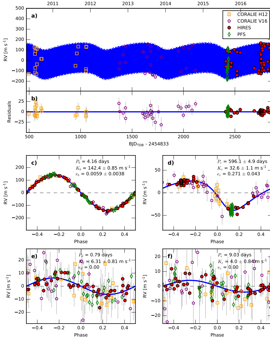
FIG. 1.— Four-planet RV model of WASP-47, assuming circular orbits for WASP-47d and WASP-47e a) The RV time-series. Filled red circles indicate Keck-HIRES data. Orange squares represent CORALIE data published by Hellier et al. (2012). Purple pentagons represent CORALIE data published by Neveu-VanMalle et al. (2016). Green diamonds indicate PFS data published by Dai et al. (2015). The solid blue line corresponds to the most likely model. Note that the orbital parameters listed in Table 2 are the median values of the posterior distributions. Error bars for each independent dataset include an RV jitter term listed in Table 2, which are added in quadrature to the measurement uncertainties. b) Residuals to the maximum-likelihood fit. c-f) The RV time-series phase folded at the orbital periods of each of the four planets after subtracting the other three planet signals.
