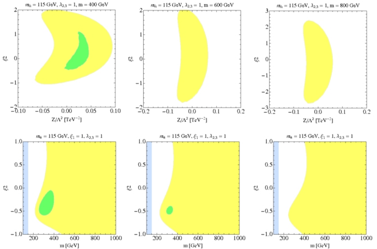
FIG. 8: Space of allowed \xi_2 and Z/\Lambda^2 for case XI_{\bar{3}} (top), left to right the masses are m_v = 400, 600, 800 \text{ GeV} , other parameters same as above, Z/\Lambda^2 same as above left to right for XI_{\bar{3}} (bottom row).
