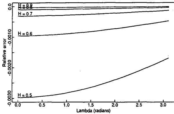
Figure 5: Relative Error in Using B_{200}(\lambda; H) Approximation.
