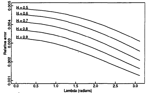
Figure 4: Relative Error in Using \tilde{B}_3(\lambda; H) Approximation.
