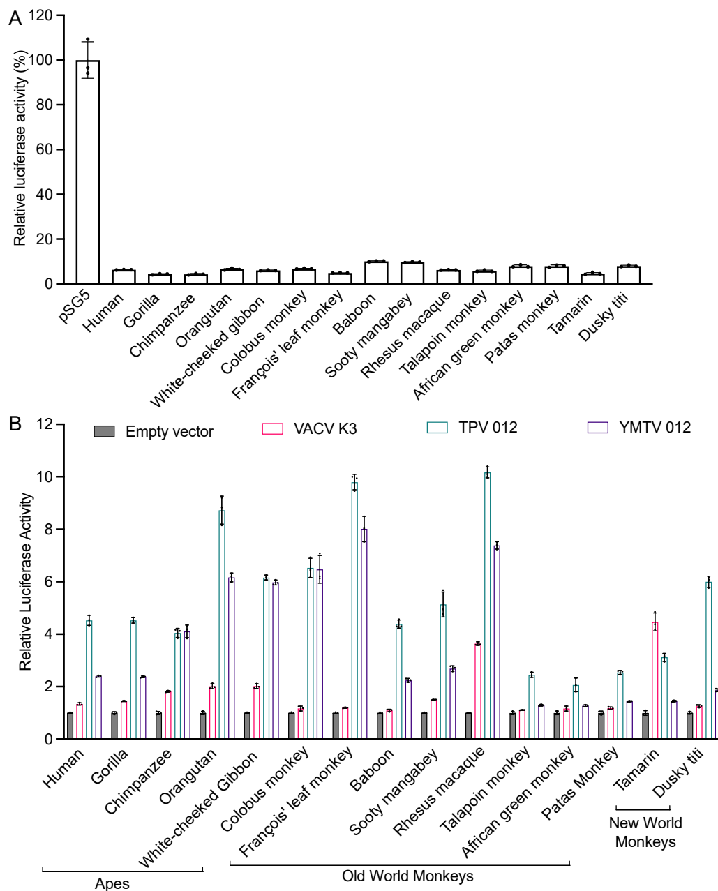
Figure 2. Differential sensitivities of tested PKRs to VACV K3, TPV 012, and YMTV 012 orthologs. (A) HeLa PKR ko cells were co-transfected with expression vectors encoding firefly luciferase (50 ng) and with either empty vector or PKR (200 ng) from the indicated species. Luciferase activities were measured 48 h after transfection and normalized to empty vector transfected cells to obtain relative luciferase activities. (B) HeLa PKR ko cells were transfected with expression vectors encoding firefly luciferase (50 ng), PKR (200 ng), and PKR inhibitor (200 ng) from the indicated species. Luciferase activities were measured 48 h after transfection and normalized to PKR-only transfected cells to obtain relative luciferase activities. Error bars represent the standard deviations from three independent transfections. The luciferase assay results shown are representative of at least three independent experiments.
