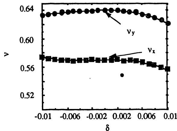
Figure 3. Tune versus energy for the test lattice which has 4 families of sextupoles, 2 in the arcs and 2 for the LCC section.
