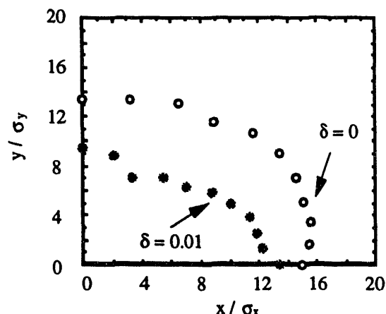
Figure 4. Initial values of particles which survived 1000 turn tracking. The open circles represent particles which were launched with zero initial energy deviation and the closed circles represent particles which had an initial energy deviation of 1%. The horizontal rms beam size, \sigma_x , was calculated assuming an uncoupled beam ( \epsilon_x = \epsilon_0 ) and the vertical rms beam size, \sigma_y , was calculated assuming a fully coupled beam ( \epsilon_y = \epsilon_0/2 ).
