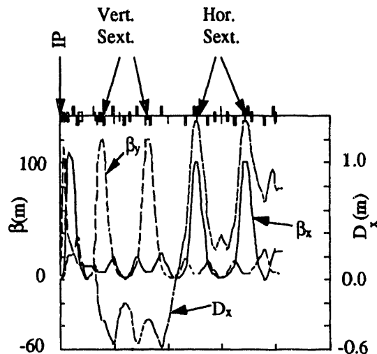
Figure 1. Lattice functions (right hand side of the IP straight) of the "test" lattice. The vertical sextupole pair and the horizontal sextupole pair follow the IP and the final doublet.
