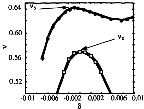
Figure 2. Tune versus energy for the reference lattice which has only 2 families of sextupoles in the arcs to correct the linear chromaticity.
