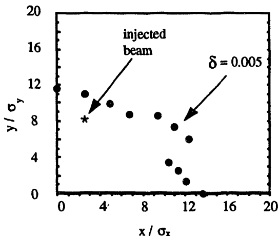
Figure 5. Particles were launched with an initial energy deviation of 0.5%. The asterisk represents the acceptance necessary for injection.
