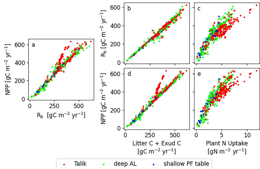
Figure 6. Plant and microbial activity are tightly coupled through exchanges of carbon and nitrogen. Annual R_h and NPP are plotted against annual carbon inputs to the soil (litter carbon + root exudate carbon) and against annual plant nitrogen uptake. Each simulation is classified into Talik (red), deep AL (green), or shallow PF table (blue) based on soil temperatures at 90 cm depth.
