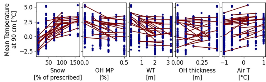
Figure 3. Responses of modeled soil temperature to factor changes are nonlinear and exhibit interaction effects. Mean annual soil temperature at 90 cm depth is plotted against the normalized snow precipitation, O-horizon macroporosity, water table depth, O-horizon thickness, and air temperature factor values for each model run (blue dots). In each subplot, the red lines link two runs associated by a change in the factor and represent the corresponding change in soil temperature. Factor descriptions and ranges can be found in Table 1.
