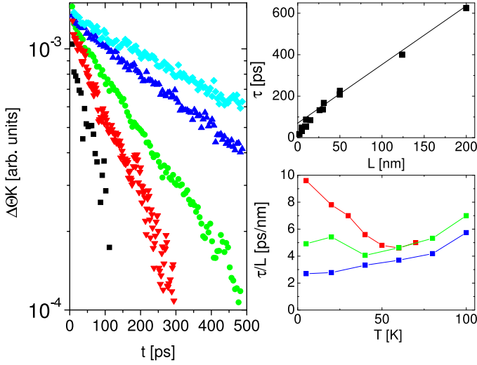
FIG. 3: (a) Semi-log plot of \Delta\Theta_K(t) for 10, 30, 50, 125, and 200 nm samples (fastest to slowest decay) (b) Decay times vs. film thickness at 10 K (c) Decay times vs. temperature for 5, 50, and 200 nm samples
