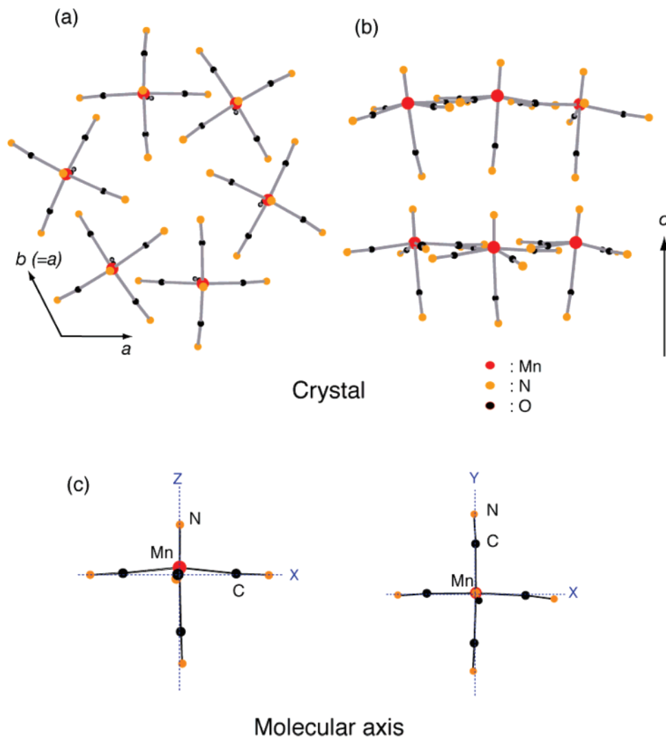
Figure 1. Crystal and molecular structures of Mn(V)-nitrido compound. (a and b) Molecular arrangement in the crystal unit cell and (c) molecular structure. The molecular z -axis (Mn≡N direction) is aligned nearly parallel to the crystal c -axis ( 9.4^\circ off). The Mn position is \sim 0.2 Å displaced out of the equatorial ligand plane toward the nitrido ligand.
