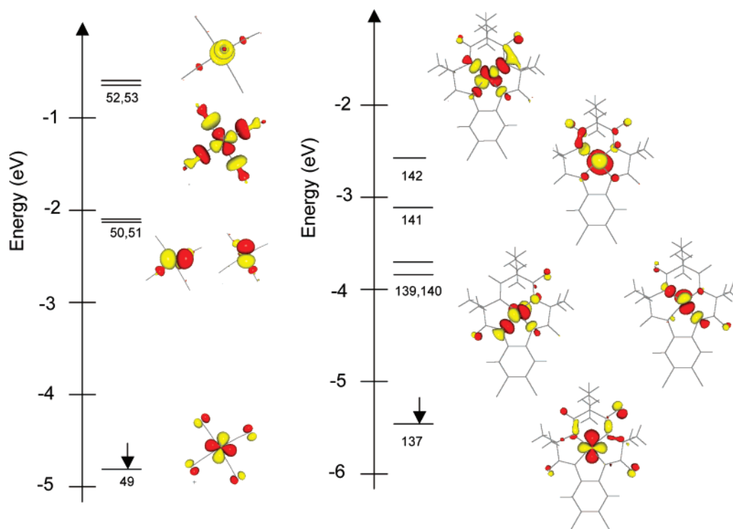
Figure 6. Spin-down molecular orbitals for the Mn(V)-nitrido (left) and Mn(V)-oxo (right) complexes.
