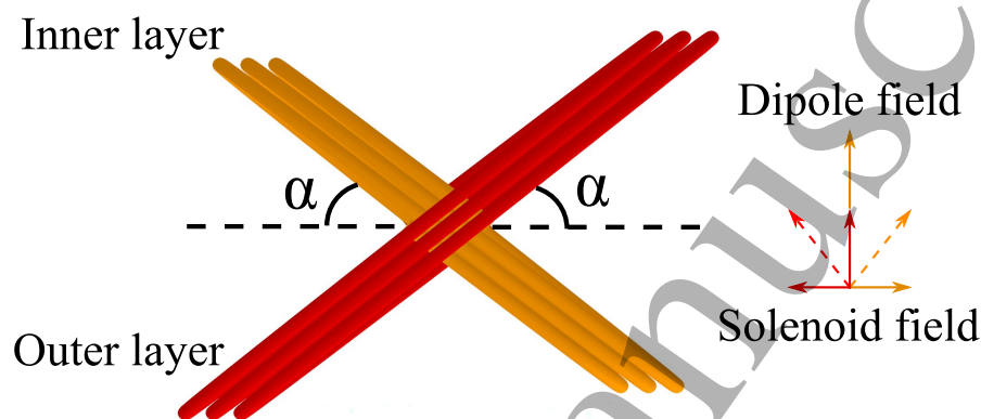
12 13 14 15 16 17 18 19 20 21 22 23 24 25 26 Figure 2. Illustration of the two-layer three-turn CCT dipole magnet 27 using CORC ® wires. The field from each layer cancels the solenoid component and 28 doubles the dipole components in the aperture. 29
