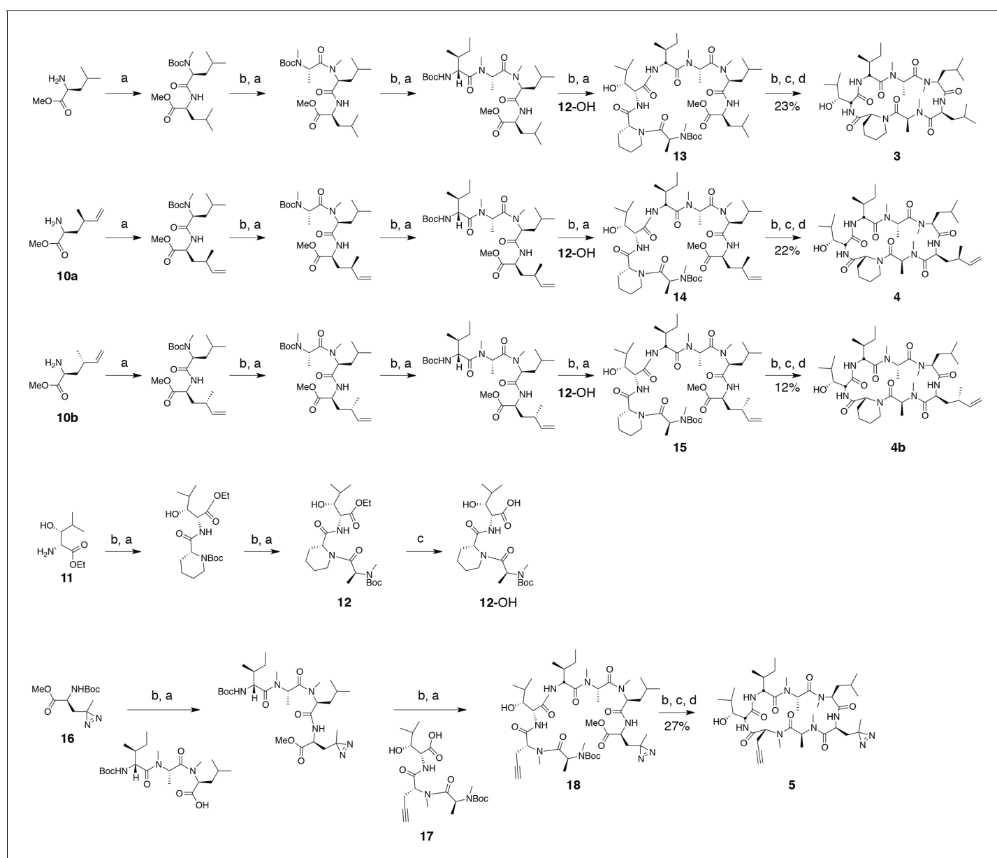
Figure 8. Synthesis of ternatin variants. Reagents and conditions: (a) HATU, DIPEA, DCM/DMF; (b) 2 M HCl, MeOH, 30^\circ\text{C} ; (c) 1 N LiOH, \text{H}_2\text{O}/\text{THF} ; (d) HATU, DIPEA, DMF.
