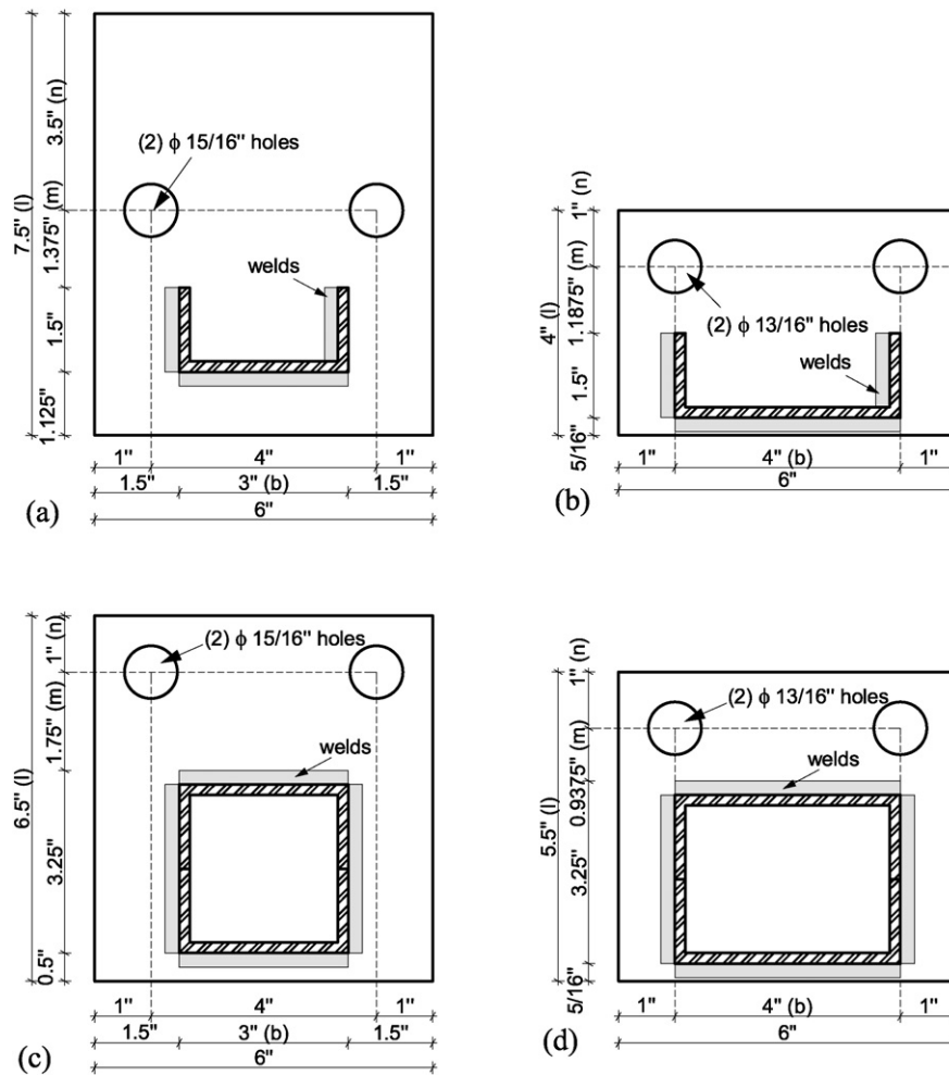
Fig. 4. Plan dimensions of the various base plate details; a-d reflect layouts A–D.
