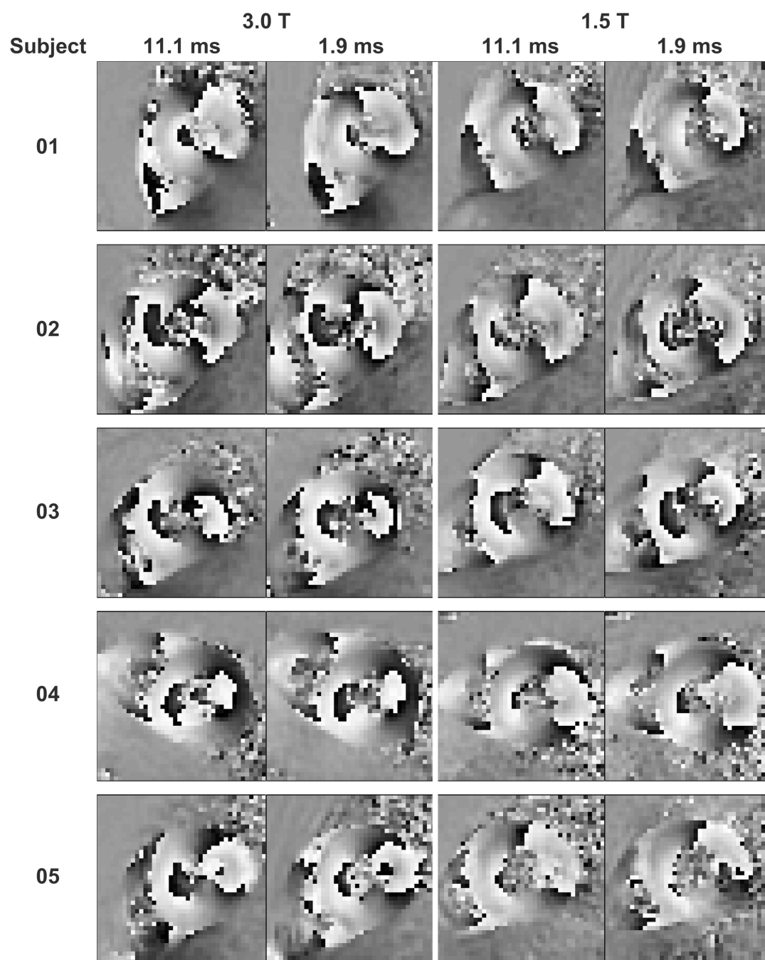
Figure 4. Phase images with displacement encoded in the x-direction were visually similar between acquisitions with 11.1 and 1.9 ms readouts. Blurring artifacts were not visually obvious in the phase images from 11.1 ms readouts.
