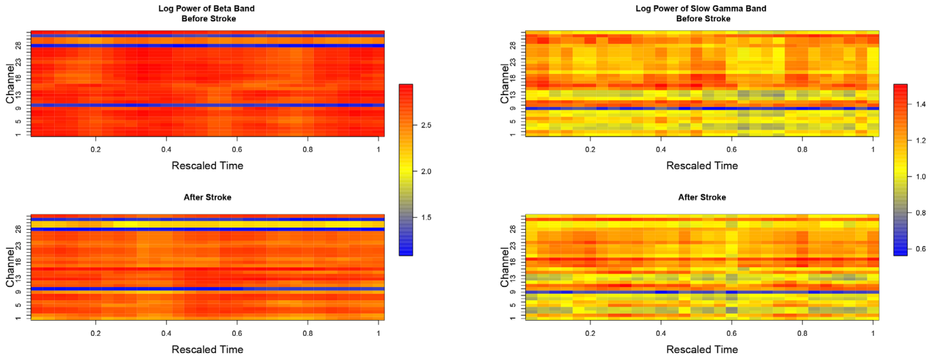
FIGURE 2 Rat stroke study: the time-frequency plot of particular frequency bands among all the microelectrodes before and after stroke. This figure appears in color in the electronic version of this article, and any mention of color refers to that version
