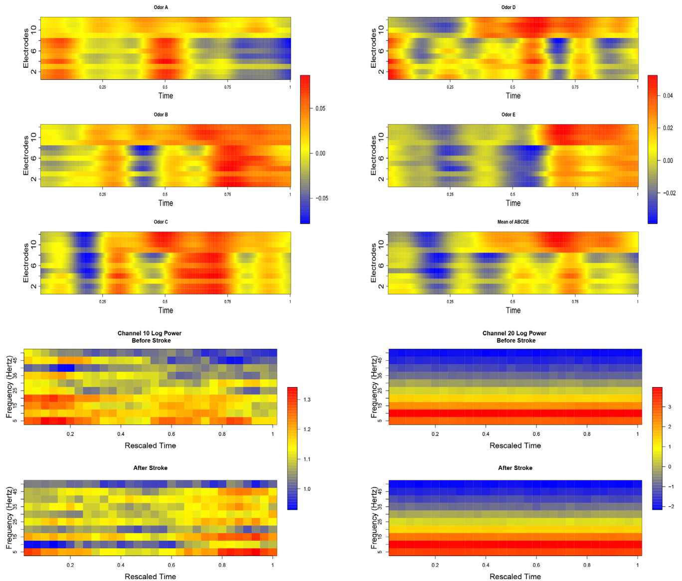
FIGURE 1 Top 6 (memory coding experiment): smoothed LFPs for odors ABCDE and their means (aggregated over all the odors) where x-axis represents rescaled time and y-axis stands for different tetrodes (channels); Bottom 4 (rat stroke study): the time-frequency plot of microelectrodes 10 and 20 among all the 600 epochs for before and after the stroke. This figure appears in color in the electronic version of this article, and any mention of color refers to that version
