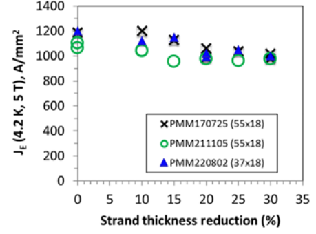
Fig. 5. J_E (4.2 K, 5 T) as a function of strand thickness reduction for three wires after 50 bar OPHT with a T_{max} of 890.5^\circ\text{C} . The J_E reduction of the rolled wires is less than 18%.
