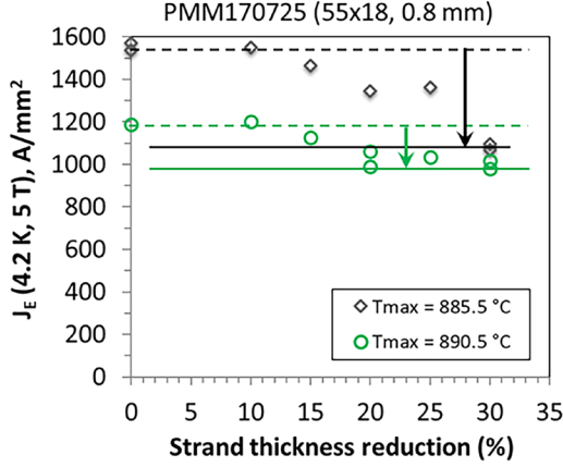
Fig. 4. J_E (4.2 K, 5 T) as a function of strand thickness reduction for wire PMM170725. The arrows from the dashed lines to the solid lines show the J_E reduction with the strand deformation. For T_{max} = 885.5^\circ\text{C} , J_E (4.2 K, 5 T) was reduced by 32%, while it reduced 18% for T_{max} = 890.5^\circ\text{C} .
