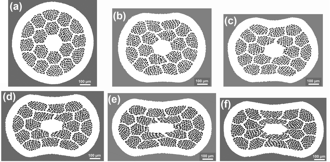
Fig. 1. Cross section images of (a) round wire, and rolled wire samples of PMM170715 (55x18, 0.8 mm) with thickness reduction of (b) 10%, (c) 15%, (d) 20%, (e) 25% and (f) 30% after 50 bar pre-densification heat treatment, 830 °C/12 hrs.
