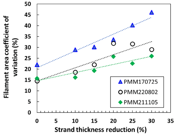
Fig. 3. Filament area coefficient of variation (CV) as a function of strand thickness reduction for wires, PMM170725 (55x18, 0.8mm), PMM220802 (37x18, 0.8 mm) and PMM211105 (55x18, 1.0 mm). The dashed trend lines are to guide the eye.
