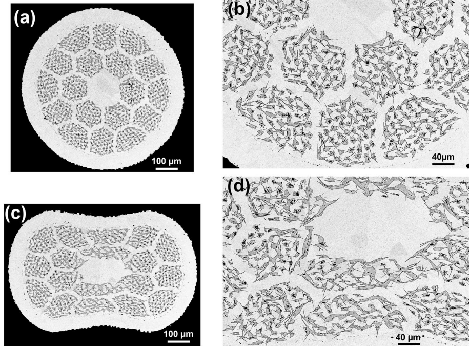
Fig. 6. SEM images of cross-sections of (a) and (b) round wire, (c) and (d) rolled wire with 20% deformation for wire PMM170725 (55x18, 0.8 mm) after 50 bar OPHT with T_{max} = 885.5^\circ\text{C} .
