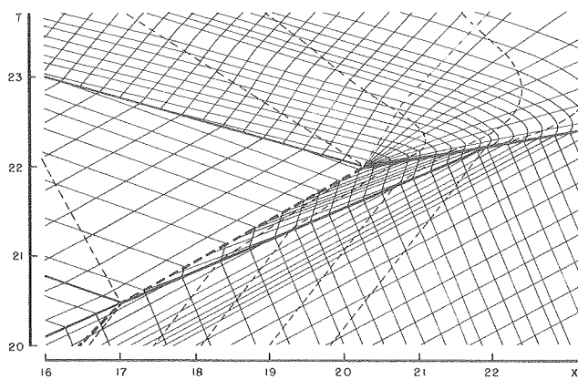
Fig. 8 Details of solution presented in Fig. 7 depicting the onset of detonation.
