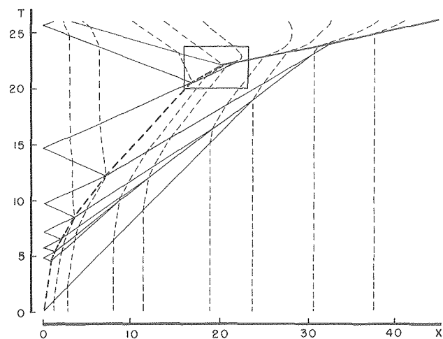
Fig. 7 Wave diagram of unstable solution obtained in the case of supercritical burning speed increment.
