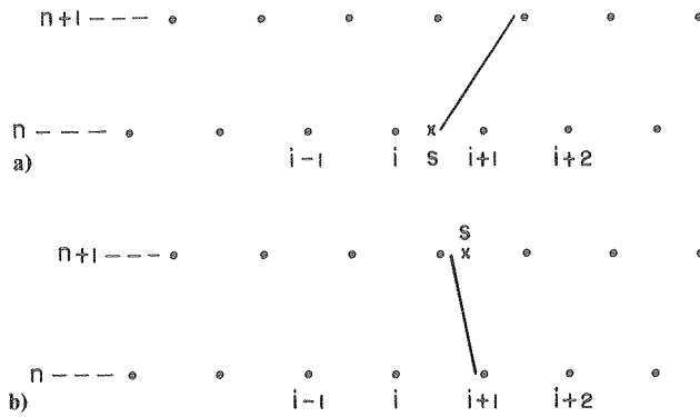
Fig. 1 Schematic diagram of shock traversing the computational grid: a) front propagating to the right; b) front propagating to the left.
