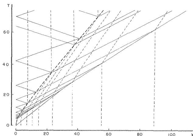
Fig. 6 Wave diagram of stable solution obtained in the case of subcritical burning speed increment.
