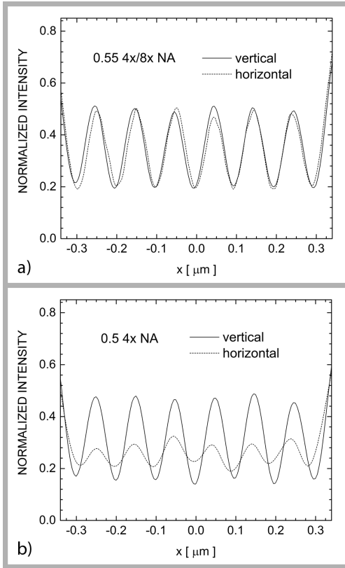
Fig. 10 Cross section of the horizontal and vertical features of the 50-nm mask CD elbows from Fig. 9, comparing (a) anamorphic imaging at 0.55 4x/8x NA (6° CRA) with (b) conventional imaging at 0.5 4xNA (8° CRA).
