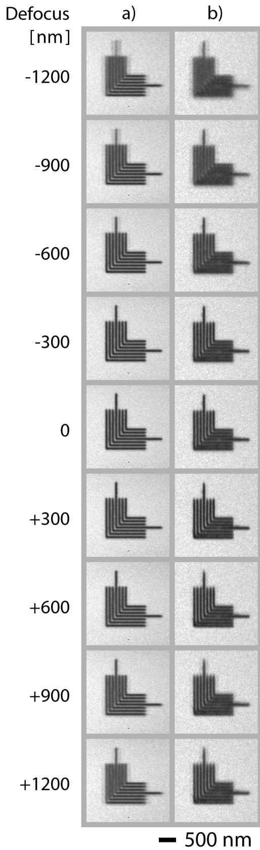
Fig. 12 Through-focus series of SHARP images, comparing through-focus behavior in (a) anamorphic imaging at 0.55 4x/8x NA (6° CRA) with (b) conventional imaging at 0.5 4xNA (8° CRA).
