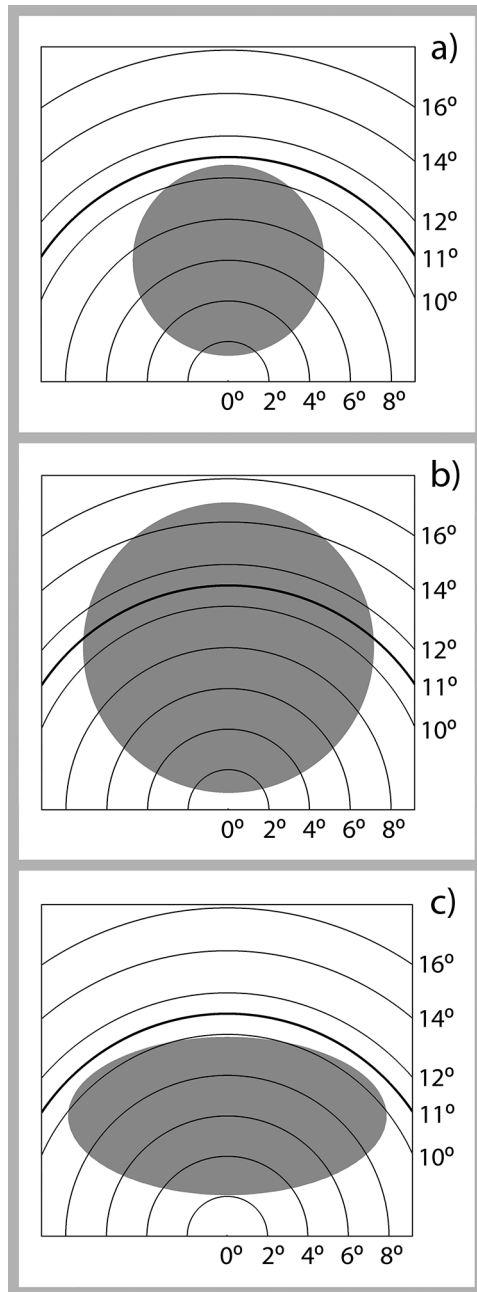
Fig. 3 Apertures of (a) a 0.33 4x NA zoneplate at 6° CRA, (b) 0.5 4x NA zoneplate at 8° CRA and (c) 0.55 4x/8x NA zoneplate for anamorphic imaging at 6° CRA in comparison and range of angles of the associated ray cones.
