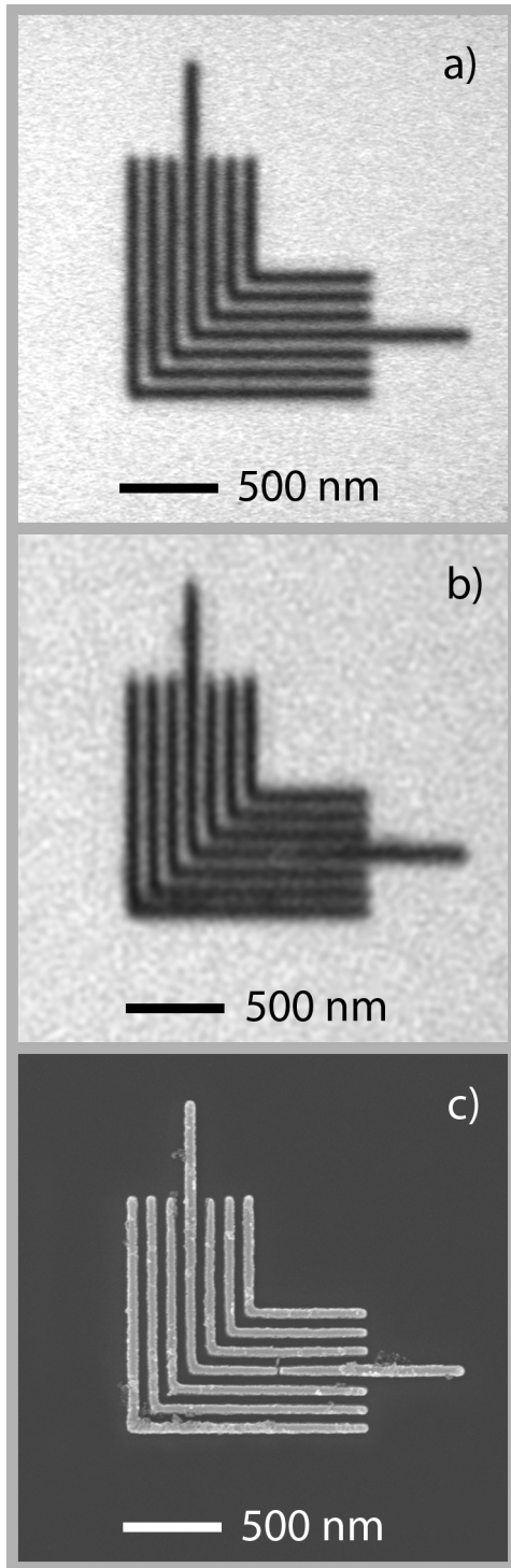
Fig. 9 SHARP aerial images of 50-nm CD elbows (mask scale), comparing (a) anamorphic imaging at 0.55 4x/8x NA (6° CRA) with (b) conventional imaging at 0.5 4xNA (8° CRA), and (c) SEM-image of the 4x elbow on the target.
