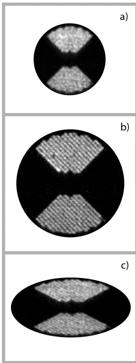
Fig. 2 Pixelated cross pole illuminator, matched to (a) the 0.33 4x NA lens at 6° CRA, (b) 0.5 4x NA lens at 8° CRA, and (c) anamorphic imaging at 0.55 4x/8x NA and 6° CRA in comparison, recorded with a YAG scintillator camera in SHARP microscope.
