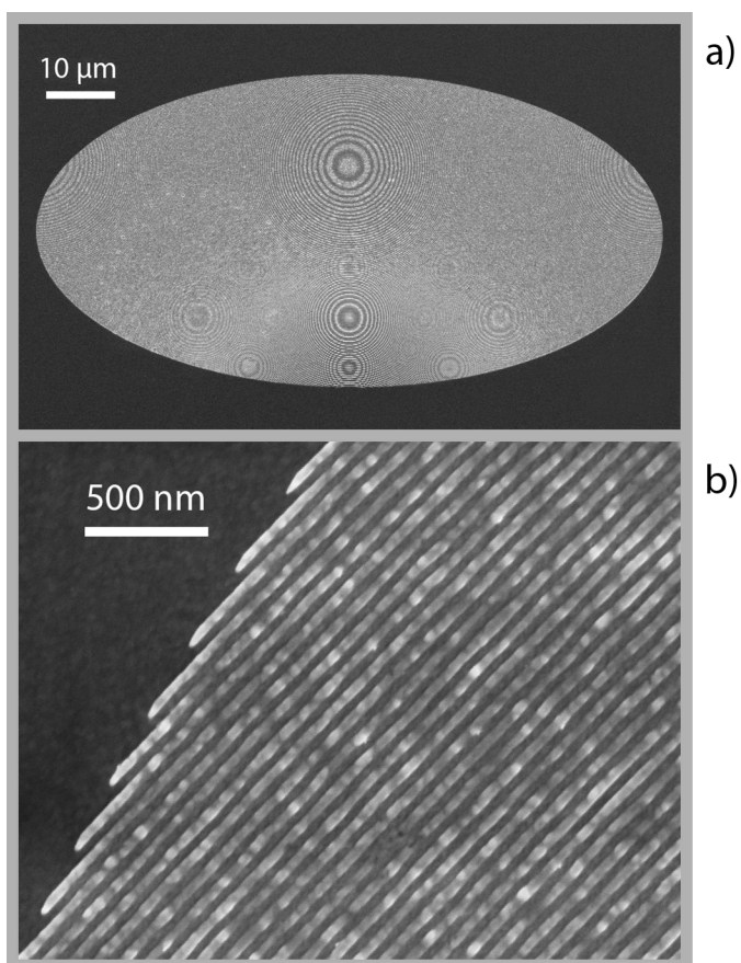
Fig. 5 SEM-image of (a) a zoneplate lens with an anamorphic aperture and (b) detail image, showing the outer zones.
