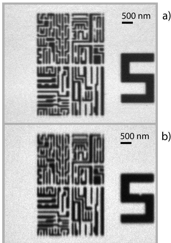
Fig. 8 SHARP aerial images of a test pattern with 50-nm CD (mask scale), comparing (a) anamorphic imaging at 0.55 4x/8x NA (6° CRA) with (b) conventional (isomorphic) imaging at 0.5 4x NA (8° CRA).
