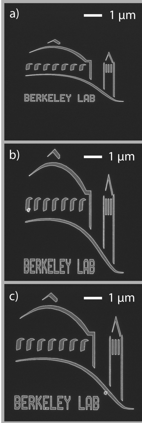
Fig. 6 SEM-images of (a) 4x reference pattern, (b) anamorphic 4x/8x, and (c) 7.5x/4.8x test patterns.
