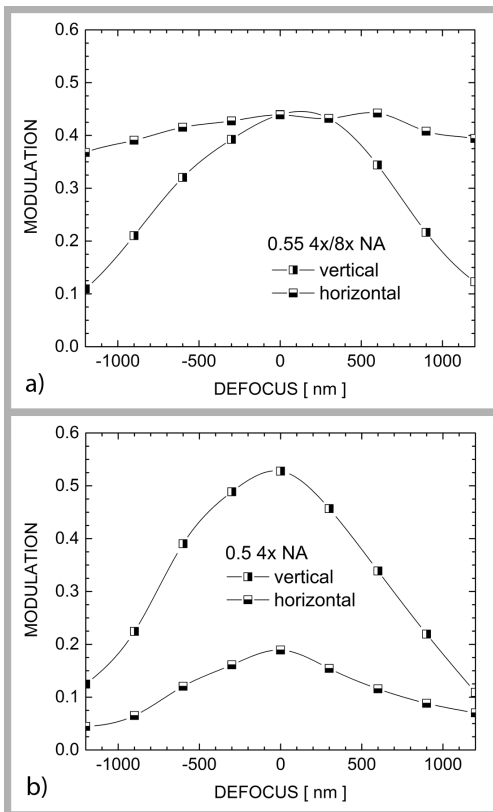
Fig. 11 Modulation of horizontal and vertical features through-focus in the (a) anamorphic, and (b) conventional series of SHARP images, shown in Fig. 12.
