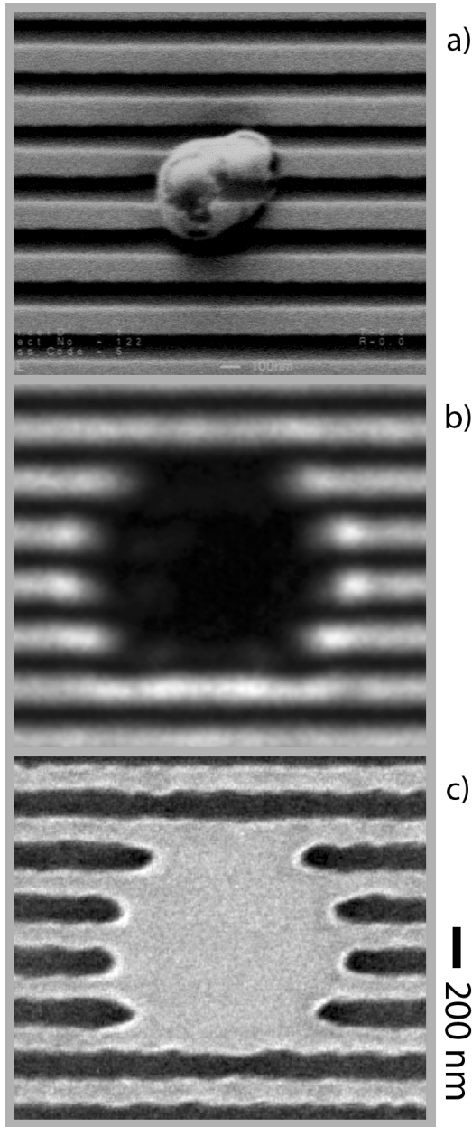
Fig. 1 Visual comparison of a large defect, 13 imaged with (a) mask-SEM, (b) SHARP EUV mask microscope, and (c) wafer-SEM.
