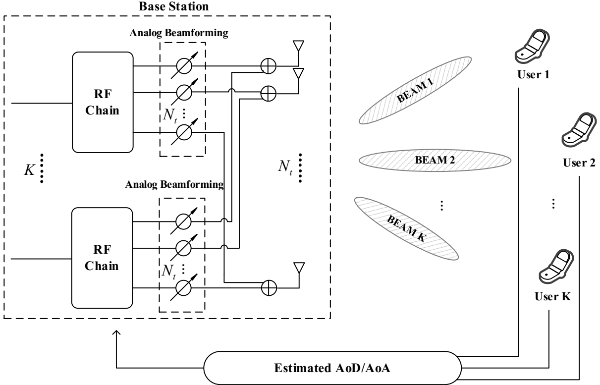
Fig. 1: System model
