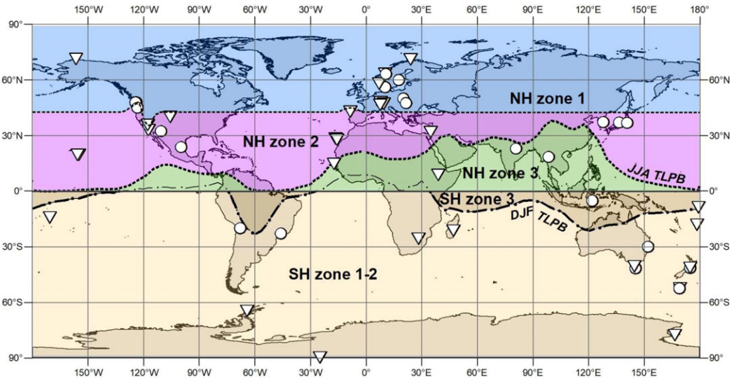
Figure 1 World map showing the zones and locations of atmospheric \text{CO}_2 sampling (triangles) for ^{14}\text{C} analysis and \Delta^{14}\text{C} tree-ring records (circles) used for our compilation. The mean positions of the TLPB during December–February (DJF) and June–August (JJA) are based on the NCEP/NCAR sea level pressure data (Kalnay et al. 1996) for 1949–2019.
